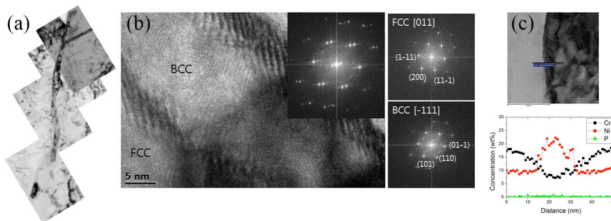
Figure 2. A Low magnified TEM image near grain boundary (a), HRTEM image and corresponding FFT images indicating the formation of BCC ( \alpha or \alpha' ) in vicinity of grain boundary (b) and EDS result showing Ni enrichment of Cr depletion in the transformed BCC ( \alpha or \alpha' ) phase.
