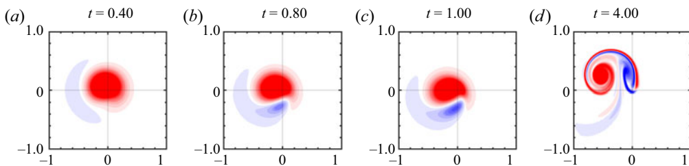
Figure 15. Time evolution of a helical vortex at L = 1.43 , a = 0.3 and Re = 10^3 with axial flow \bar{W}_B = 4.0 (above the threshold). Contours are as in figure 14.
