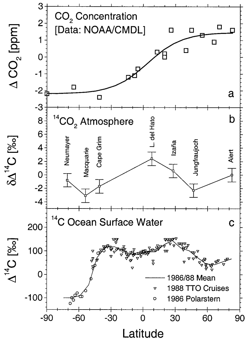
Figure 3 Mean meridional profiles 1993–1994 of (a) \text{CO}_2 concentration (data from the NOAA/CMDL global network [Tans et al. 1996]) and (b) \Delta^{14}\text{C} in the atmosphere (Heidelberg unpublished data). Plotted are in (a) and (b) the deviations \Delta\text{CO}_2 and \delta\Delta^{14}\text{C} from the global mean values. (c) \Delta^{14}\text{C} of DIC in surface ocean water derived from cruises of the TTO experiment (Broecker et al. 1995) together with unpublished Heidelberg data collected in 1986 in the South Atlantic ocean during the Polarstern cruise ANT III. The solid line represents a spline through the 1986/1988 data.
