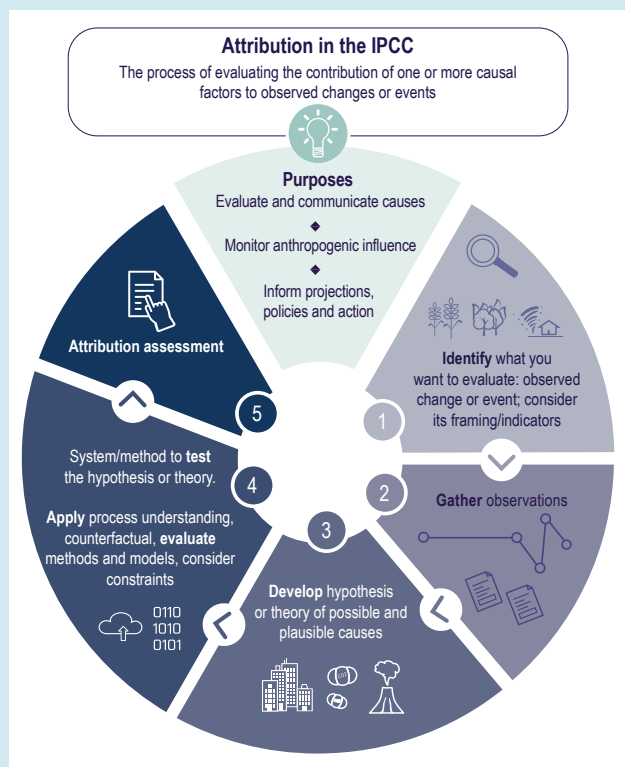
Cross-Working Group Box: Attribution, Figure 1 | Schematic of the steps to develop an attribution assessment, and the purposes of such assessments. Methods and systems used to test the attribution hypothesis or theory include: model-based fingerprinting; other model-based methods; evidence-based fingerprinting; process-based approaches; empirical or decomposition methods; and the use of multiple lines of evidence. Many of the methods are based on the comparison of the observed state of a system to a hypothetical counterfactual world that does not include the driver of interest to help estimate the causes of the observed response.
