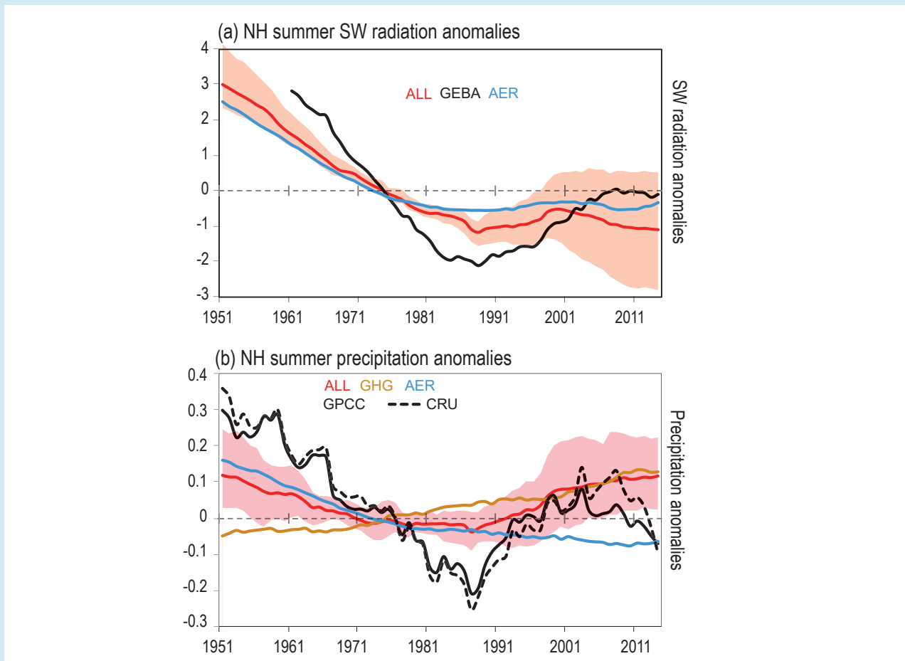
Box 8.1, Figure 1 | Northern Hemisphere surface downward radiation anomalies ( W m^{-2} ; a) and precipitation anomalies ( mm day^{-1} ; b) for 1951–2014 for summer season (May–September) monsoon region (Polson et al., 2014) from CMIP6 DAMIP experiments. Observed solar radiation anomalies are from GEBA global data from 1961–2014 (Wild et al., 2017) and observed precipitation anomalies are from GPCC and CRU. CMIP6 multi-model mean anomalies are from all-forcings (ALL), greenhouse gas forcing (GHG) and anthropogenic aerosol forcing (AER) experiments. Anomalies are with respect to 1961–1990 and smoothed with a 11-year running mean. Red shading shows the ensemble spread of ALL forcing experiment (5–95% range). Models are masked to the GPCC data set. Further details on data sources and processing are available in the chapter data table (Table 8.SM.1).
