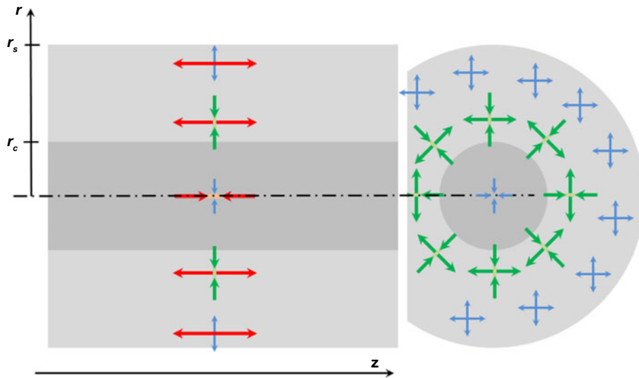
Fig. 1. Strain distribution in a cylindrical core-shell NW. Arrows indicate the longitudinal strain (in red), the inhomogeneous shear strain in the shell (in green), and the rest of the strain – uniform and isotropic in the plane (in blue). The lattice parameter is assumed to be smaller in the shell than in the core ( f < 0 ).
