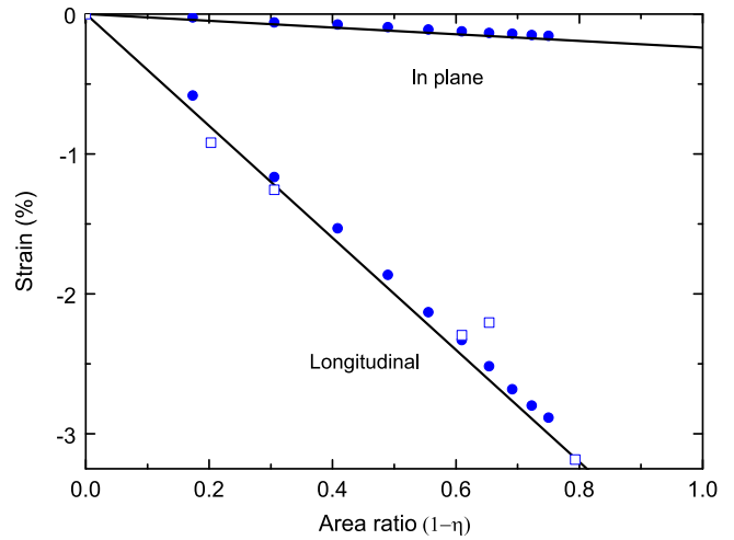
Fig. 2. Strain in the core of a GaN-AlN NW, as a function of the area ratio. Solid symbols, microscopic calculation, open symbols, electron microscopy data, both from reference [17]; lines, present calculation.
