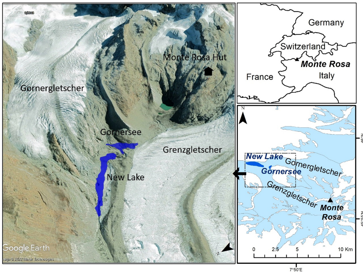
Fig. 1. Google Earth image shows the study area with Gornerssee and surrounding areas of the western declivity of the Monte Rosa massif.
