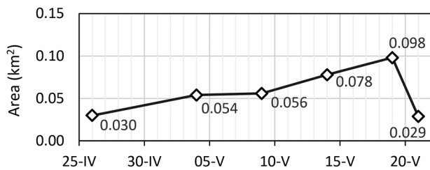
Fig. 3. Growth and drainage of the new lake near Grenzletscher in April and May 2022 as documented by changes in area derived from satellite images.
