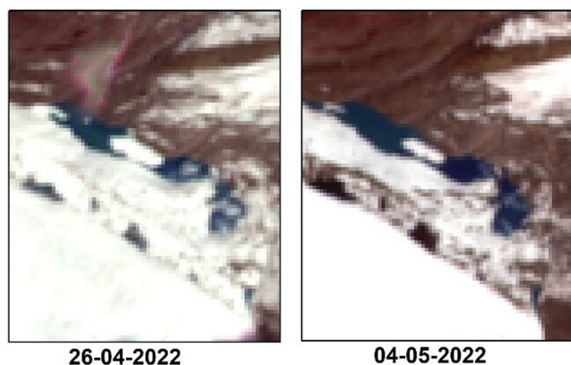
Fig. 2. Evolution of the lake near Grenzgletscher on false colour composite (FCC) images using bands 8, 4 and 3 of Sentinel-2 satellite data.
