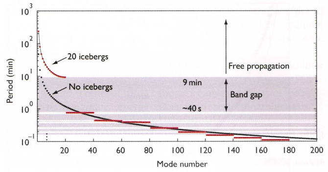
Fig. 2. Periods of barotropic seiches on the density interface of the fjord. The spectrum in the presence of 20 icebergs is compared with the spectrum in which no icebergs are present. The effects of the icebergs are to substantially lengthen the periodicity of the most fundamental normal modes (seiches with largest length scales) and to introduce band gaps below \sim 9 min. Excitation in the fjord with period < 9 min will not propagate as a free wave, but will exist as a trapped (evanescent) oscillation near the source of excitation. Below \sim 40 s period, there are many regions of propagating modes and band gaps. These regions correspond to seiches localized in the fjord segments between individual icebergs. We emphasize that this spectrum was computed to illustrate the possible influence of ice melange, and that other quantitative and qualitative effects are possible if the characterization of the ice melange is changed.
