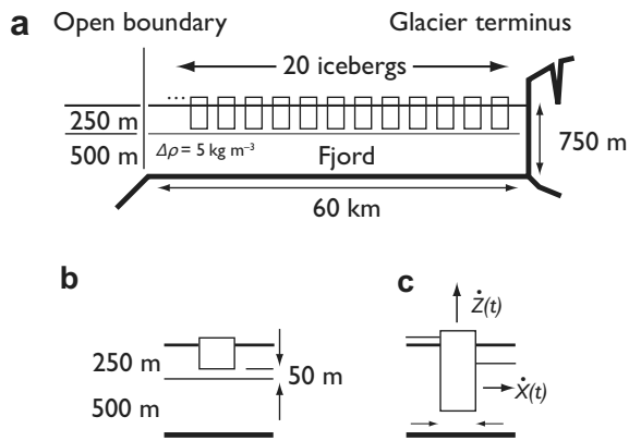
Fig. 1. Geometry of an idealized fjord containing icebergs for which seich periods are computed. (a) The two-dimensional cross section of the domain on which normal modes are computed. The 60 km long fjord is 750 m deep, closed at one end by a vertical glacier terminus, and connected to an open ocean at the other end. Ice melange is represented by filling the fjord with 20 discrete icebergs that are spaced evenly along the length of the fjord. The fjord is assumed to possess a two-layer density structure with a density interface (across which the density varies by 5 \text{ kg m}^{-3} ) that separates a relatively fresh layer (250 m thick) from a relatively salty layer (500 m thick). (b) Internal modes are computed by assuming an iceberg draft of 200 m, that reduces the upper density layer thickness from 250 m to 50 m in segments of the fjord in which icebergs float. (c) External, barotropic modes are computed for the free surface (water/air interface) of the fjord, assuming that the combined iceberg/ocean system has two degrees of freedom in the segments of the fjord where icebergs float. The two degrees of freedom are vertical heave, \dot{Z} , and horizontal surge, \dot{X} .
