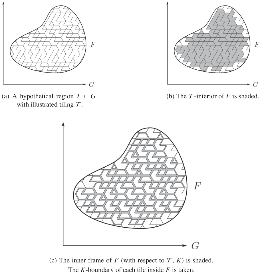
FIGURE 1. A sketch of the construction of \text{fr}_{\mathcal{T},K}(F) .
