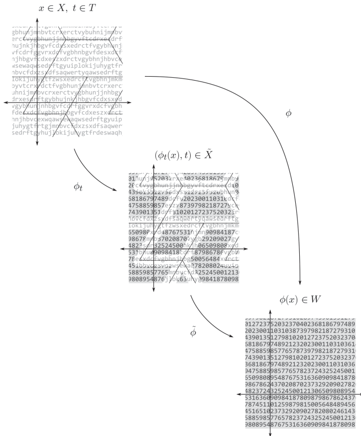
FIGURE 3. A hypothetical point x \in X with a tiling t \in T overlaid; the partially transformed point \phi_t(x) is pictured, which is labeled with symbols from both X and W ; finally, the wholly transformed image point \phi(x) \in W is reached.
