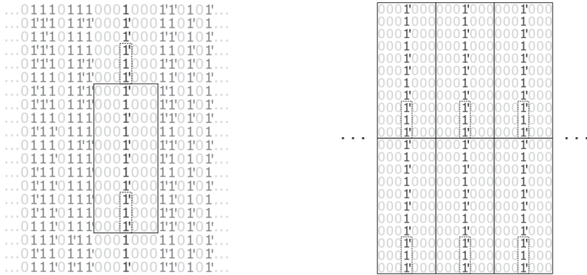
(a) A hypothetical point z is illustrated around [-n, n] \times [\ell_1, \ell_2] . The repeated vertical word \zeta is indicated by the dotted box, and the rectangle r by the solid box.
