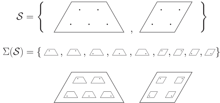
FIGURE 2. A hypothetical collection of shapes \mathcal{S} , the appropriate alphabet \Sigma(\mathcal{S}) , and (the \mathcal{T} -layer of) two aligned blocks are pictured. Each point of each block is labeled with the correct shape type and relative displacement within that shape.
