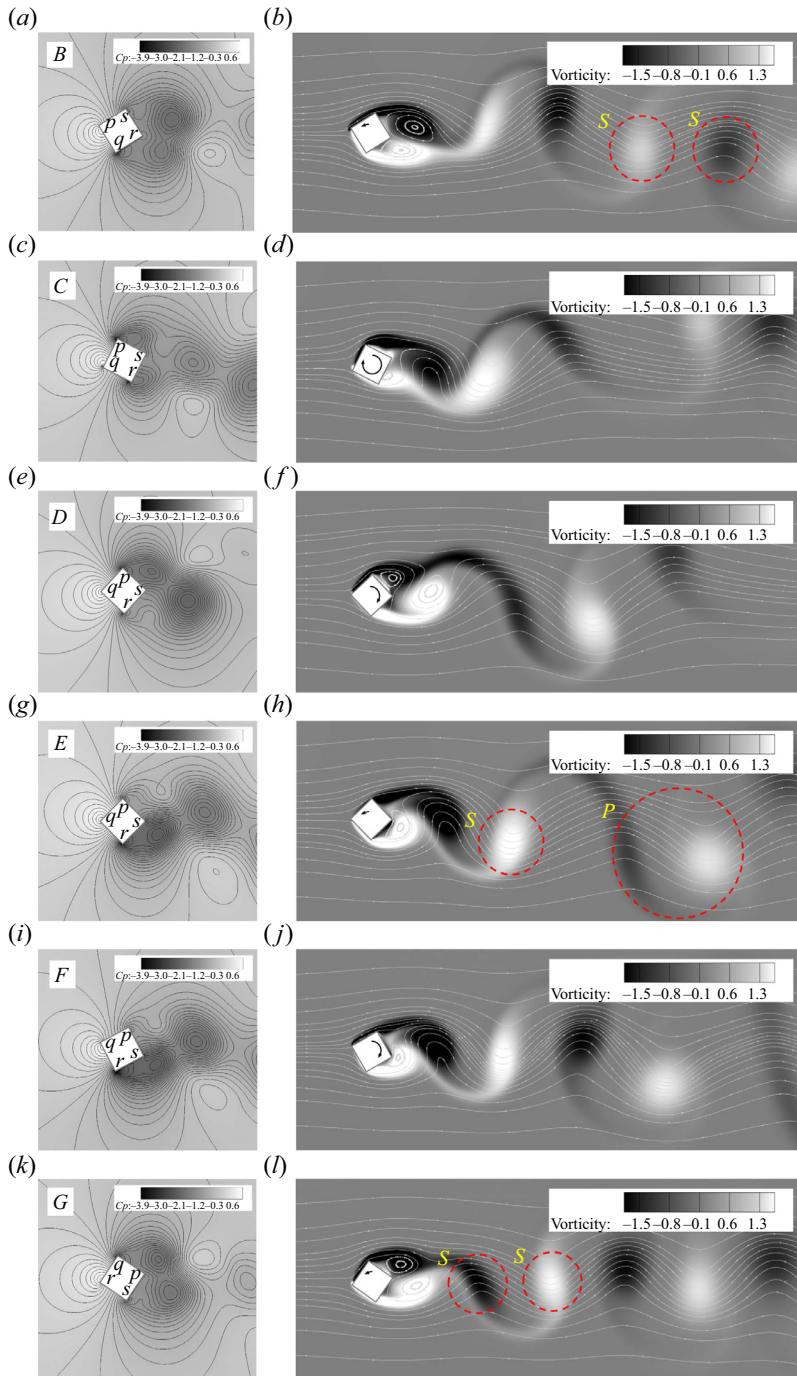
Figure 8. Pressure contours ( a,c,e,g,i,k ) and streamlines with spanwise vorticity contours ( b,d,f,h,j,l ) for the transition regime at six instants ( B to G ) marked in figure 7. The arrow inside the cylinder represents the angular velocity of cylinder.
