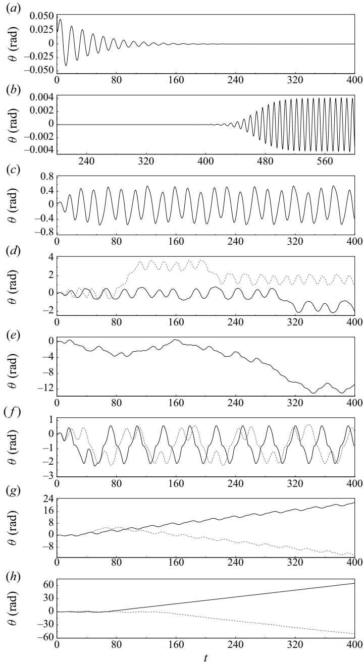
Figure 3. Time histories of rotation angle of typical regimes: (a) stable regime ( Re = 40, \rho = 2 ); (b) small-amplitude oscillation regime ( Re = 70, \rho = 10 ); (c) \pi/2 -limit oscillation regime ( Re = 80, \rho = 2 ); (d) transition regime (solid line, Re = 90, \rho = 4 ; dashed line, Re = 100, \rho = 1 ); (e) random rotation regime ( Re = 100, \rho = 2 ); (f) \pi -limit oscillation regime (solid line (1-peak subregime), Re = 130, \rho = 1 ; dashed line (2-peak subregime), Re = 140, \rho = 3.1 ); (g) wavy rotation regime (solid line, Re = 140, \rho = 2.5 ; dashed line, Re = 140, \rho = 2.6 ); (h) autorotation regime (solid line, Re = 150, \rho = 2 ; dashed line, Re = 150, \rho = 0.1 ).
