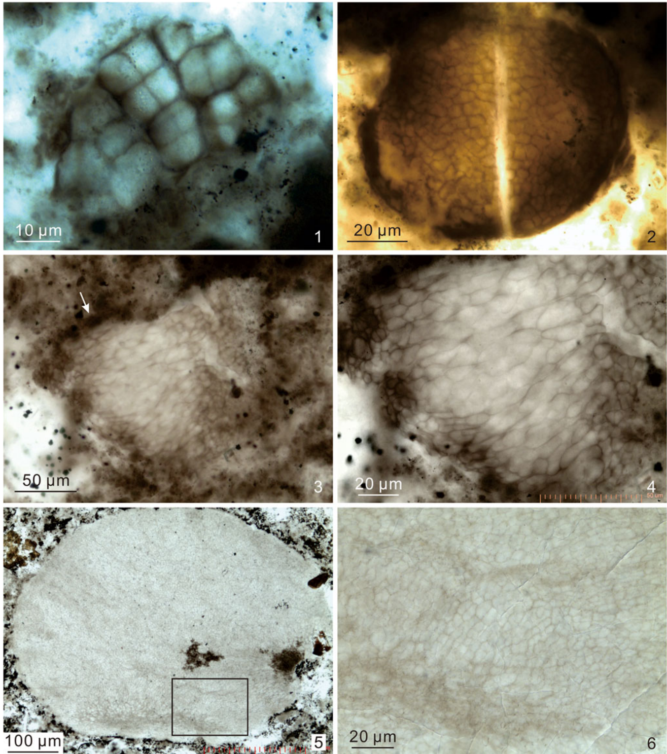
Figure 33. Multicellular algae. (1) Sarcinophycus radiatus Xiao and Knoll, 1999, DH-14-52.6-B, 13.6 × 120.5, EF-O20-2, VPIGM-4828; (2) Wengania minuta Xiao, 2004, S4-4-F2-13-A, 11.8 × 127.0, EF-Q26-4, VPIGM-4908; (3, 4) Thallophycoides phloeatus Zhang and Yuan, 1992, DH-14-68.0-A-2, 7.3 × 112.0, EF-V12, VPIGM-4863, arrow in (3) marks area magnified in (4); (5, 6) Wengania exquisita Zhang et al., 1998, S4-4-F2-5, 24.1 × 102.7, EF-D3-3, VPIGM-4879, rectangle in (5) marks area magnified in (6).
