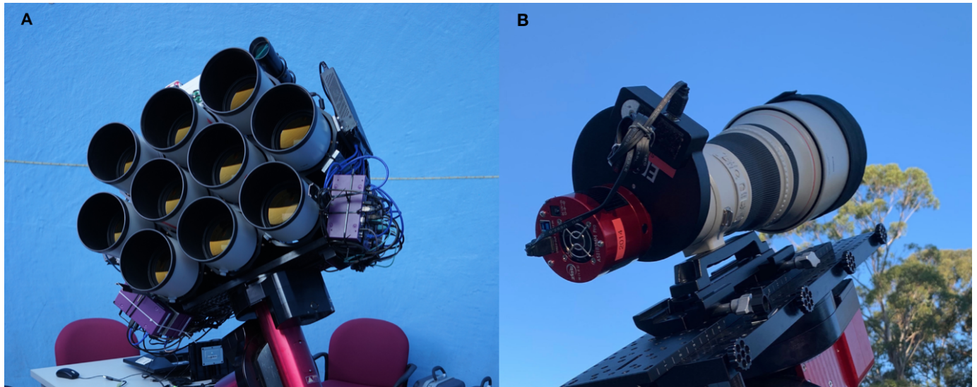
Figure 2. A) The Huntsman Telescope remote observing facility located at Siding Spring Observatory, Australia. The telescope consists of 10 Canon 400 mm f/2.8 lenses in an array configured to cover the same field of view of 1.89^\circ \times 1.26^\circ with a pixel scale of 1.24'' . B) The pathfinder instrument used to test daytime observing modes for this work consisting of a single lens. The unit is located at Macquarie University Observatory, Sydney, Australia
