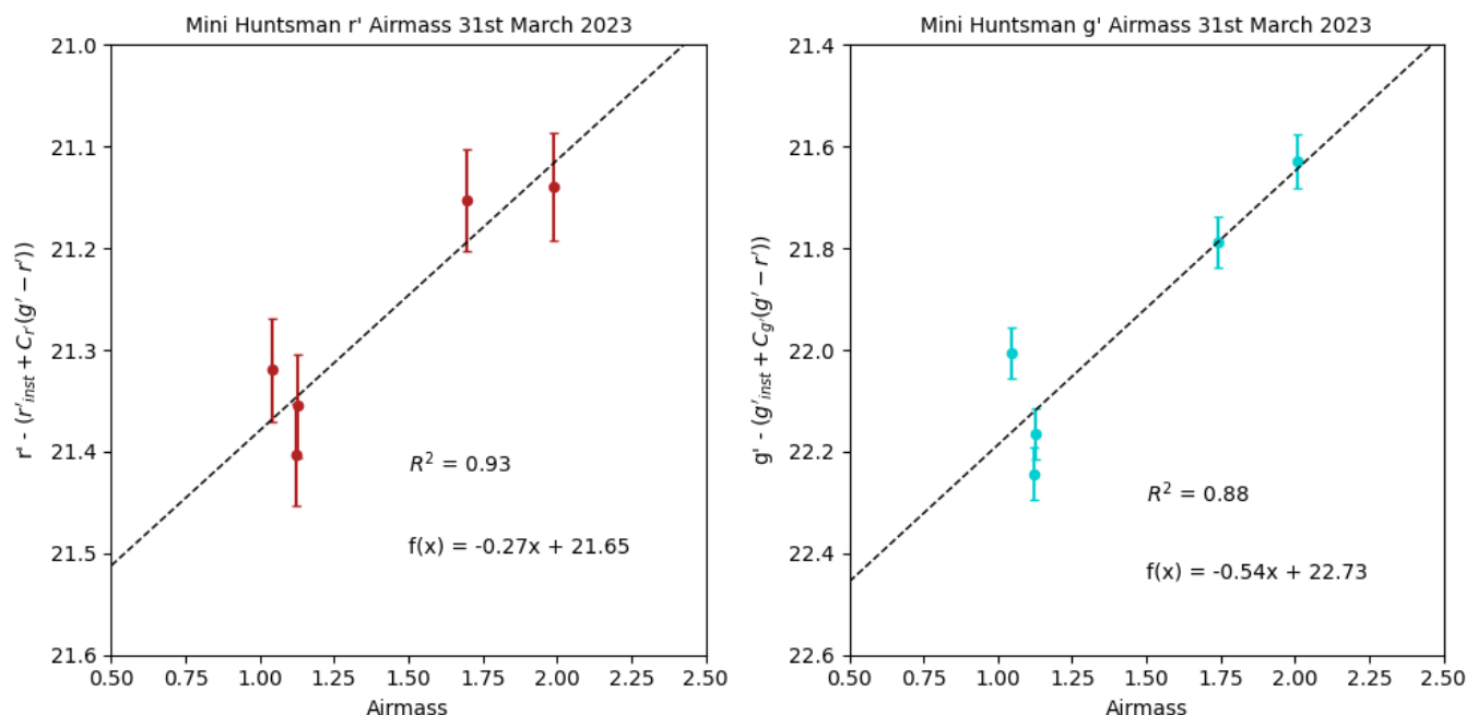
Figure 4. An example airmass plot for the 31st of March 2023, showing the calculated magnitude as a function of airmass for 5 bright reference stars. Observing logs show a clear day, no wind, with tops of 25^{\circ}\text{C} ( 77^{\circ}\text{F} ). Each data point is the median of a set of 1000 exposures for that reference star. The extinction coefficient for this day is found to be 0.27 for r' and 0.54 for g' with zeropoints of 21.65 and 22.73 respectively. The error bars encapsulate the statistical error of the set of 1000 observations, and the flat field error in quadrature. The Chi squared values for the linear fit are calculated to illustrate the fit, with a higher Chi squared of 0.93 for r' as opposed to g' . Scatter about an airmass of 1 may be due to dust in the air produced by lawn mowing that observing logs showed to occur close to the observatory at the time of observations.
