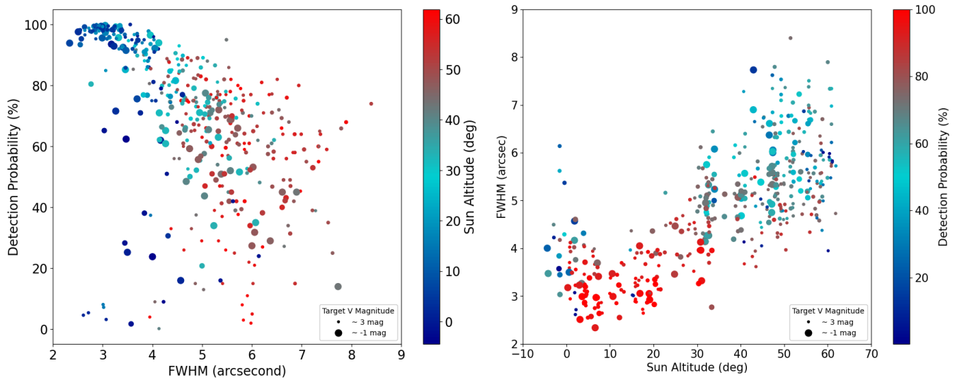
Figure 8. Left panel: The detection probability as a function of the measured FWHM, with colour bar as the Sun altitude in degrees at the time of observation, and the target magnitude is the relative size of the data points. Detection probability is show to decrease with increased FWHM corresponding to the local seeing conditions, and Sun altitude. Right panel: We plot the FWHM as a function of the Sun altitude with detection probability as the colour bar. the We see a relationship between the FWHM and the detection probability, with observations at a detection rate greater than 80% occurring in majority below a FWHM of 4 arcseconds, and a Sun altitude of 30 degrees.
