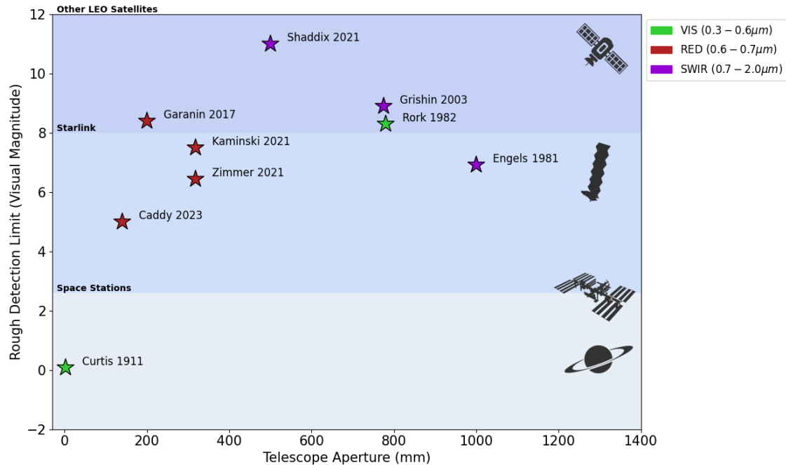
Figure 1. A sample of detection limits for visual (green), red (red), and short wave infrared (SWIR) (purple) presented in the literature for daytime observations of stars. The data included is from the works of Curtis 1911; Engels et al. 1981; Rork, Lin, and Yakutis 1982; Grishin, Melkov, and Milovidov 2003; Garanin et al. 2017; Kamiński et al. 2021; Shaddix et al. 2021; Zimmer, McGraw, and Ackermann 2021 and this work. Only works that explicitly mention a detection limit are included. Due to the lack of public information surrounding some of the hardware used in daytime observing by various research groups, a reliably reported parameter of telescope aperture is plotted against the detection limit. It should be noted that each of these instruments likely have very different focal lengths and other characteristics, as well as different data reduction methods that may bias results. Three shaded regions in visual magnitudes are also presented, showing rough predicted and observed magnitude lower margins during the day. The brightest stars and planets are visible to most optical systems including the eye (Curtis 1911) during the day, and are around \sim 0 th magnitude. The International Space Station has been observed to have a visual magnitude during the day of \sim 2 nd magnitude at zenith (this work). Starlink satellites have been observed in the day up to 3.0 mag (Halferty et al. 2022) at night, and up to 2.6 mag during the day (Zimmer, McGraw, and Ackermann 2021). Following the work of Kamiński et al. 2021, most other LEO satellites have a visual magnitude fainter than 8th magnitude.
