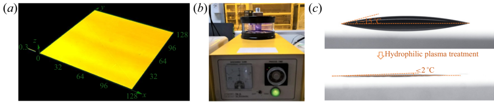
Figure 14. (a) Characterization of the glass substrate ( S_q = 0.012 \mu\text{m} ), (b) plasma treatment and (c) wettability characterization with a pure water droplet on slide glasses before and after the plasma treatment.
