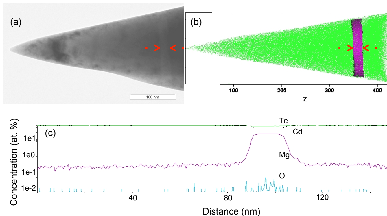
Figure 2. (a) Transmission electron micrograph of epitaxially grown CdTe with a \sim 21 nm CdMgTe heterojunction. (b) APT reconstruction of same sample using Mg isoconcentration surface. The green points are Te (c) Concentration of Cd, Te, Mg, and O across the CdMgTe heterojunction layer.
