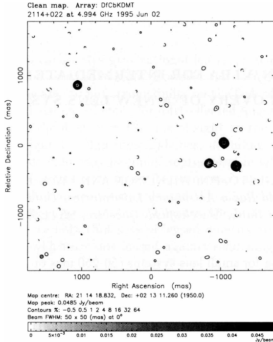
Figure 1. MERLIN map of 2114+022 at 5 GHz (11hrs. phase-referencing). The noise level is very low ( < 0.1 mJy) and there are no signs of any extended structure; all the four images are unresolved. The (variable?) fluxes of the components are, starting from the east (left): 20 mJy (21 mJy - snapshot 10 days after), 13 mJy (10 mJy), 50 mJy (45 mJy), 66 mJy (60 mJy); the spectral indexes are: \alpha_{1.6-5} = 0.32 and \alpha_{5-8.4} = 0.95 , \alpha_{1.6-5} = -0.30 and \alpha_{5-8.4} = -0.87 , \alpha_{1.6-5} = -0.65 and \alpha_{5-8.4} = 0.42 , \alpha_{1.6-5} = 0.03 and \alpha_{5-8.4} = 0.78 . The optical identification (POSS) - 19 m elliptical red “blob” (optical counter-parts?) - is only 21° misaligned with the NE-SW radio-alignment.
