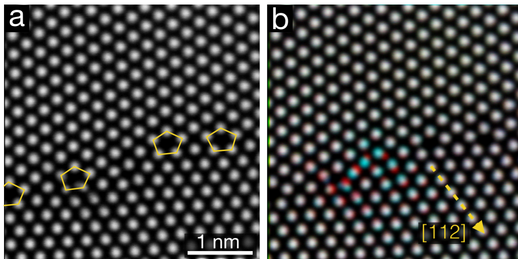
Figure 1: (a) Intensity average of 40 HAADF-STEM fast scan ( 0.5\mu\text{s} dwell time) images showing an incommensurate boundary segment containing two steps. Five-fold structural units are outlined in yellow. (b) RGB overlay of averaged intensities before, during, and after a structural event to highlight the atomic displacements.
