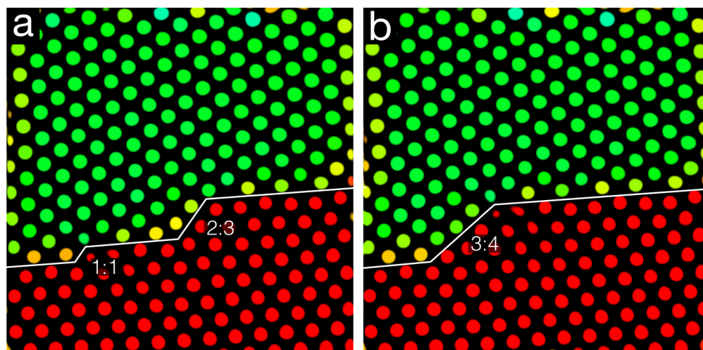
Figure 2: Grain boundary structure before (a) and after (b) collective rearrangement, colored by local coordination. Green and red correspond to the unique grain orientations, while yellow and orange show local distortions near the boundary. The boundary is highlighted for clarity.
