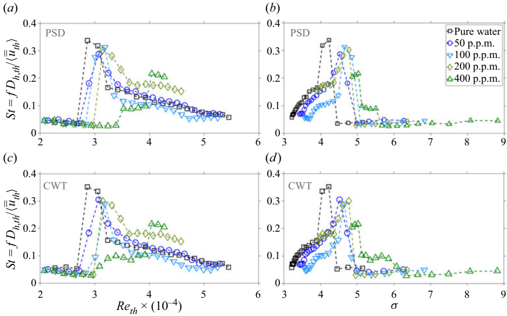
Figure 19. Throat hydraulic diameter D_{h,th} based Strouhal number St (see (3.2)) as a function of (a) the throat Reynolds number Re_{th} , and (b) cavitation number \sigma in pure water and different PAM solution flows. Panels (a,b) and (c,d) display the results of PSD and CWT spectral analysis, respectively.
