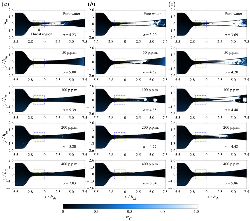
Figure 12. Snapshots of instantaneous vapour ratio fields in different PAM solution flows at the convergence and throat regions for (a) Re_{th} = 2.6 \times 10^4 , (b) Re_{th} = 3.0 \times 10^4 and (c) Re_{th} = 3.4 \times 10^4 , projected on the channel's midspan (plane z = 0 ). The white colour ( \alpha_G = 1 ) shows the cavitation areas, and the black colour ( \alpha_G = 0 ) demonstrates the bulk liquid. The flow direction is from left to right and a pale-yellow rectangle, with dashed blue borders, signifies the throat region on each figure. For sample videos, refer to movies 7–8.
