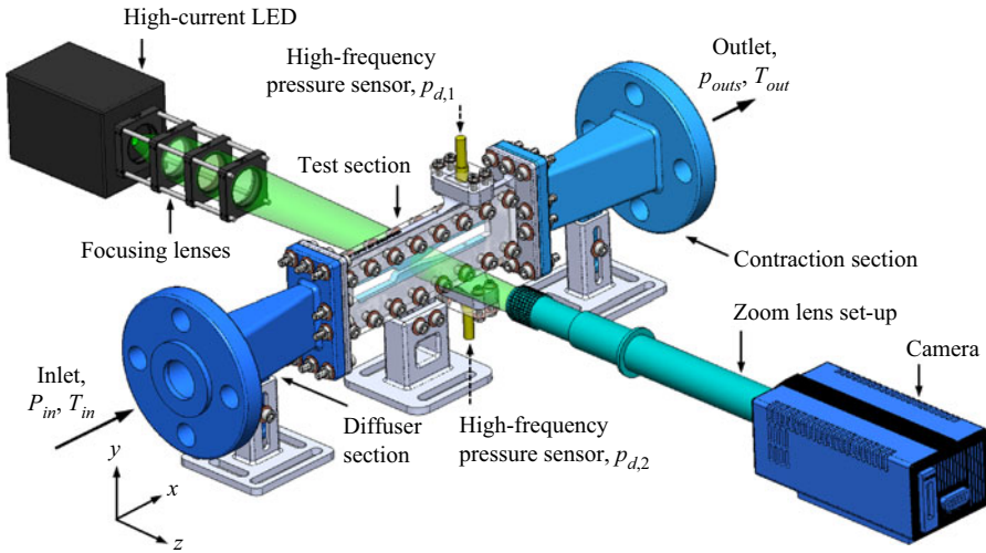
Figure 3. Backlit illuminated optical set-up to visualize the flow. The high-current LED was equipped with biconvex lenses to focus the light beams and a diffuser to distribute them uniformly in the region of interest.
