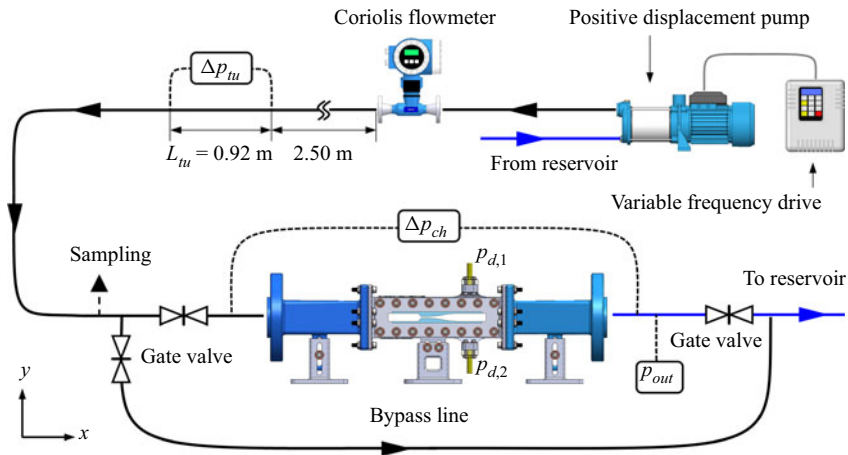
Figure 1. Schematic representation of the flow loop and its main components (not to scale).
