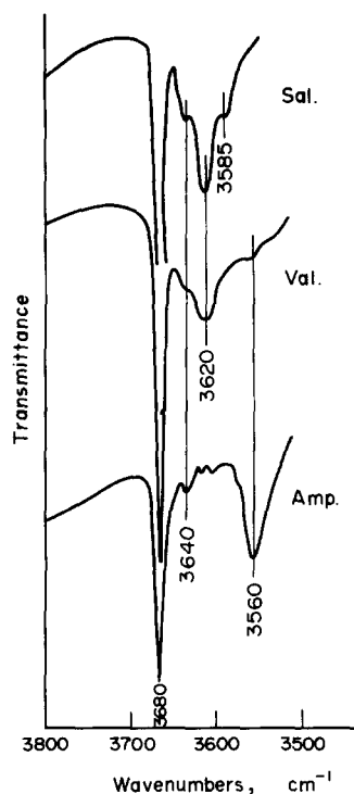
Fig. 6. Infra-red spectra of three sepiolites after deuteration at temperatures up to 140°C; Salinelles (Sal), Vallecas (Val), Ampandrandava (Amp).
