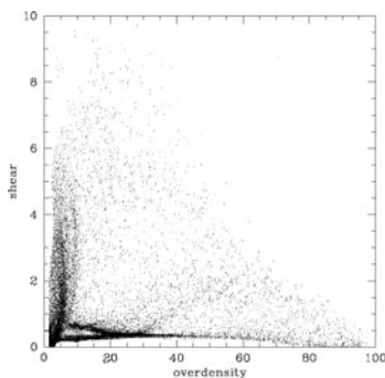
Figure 2. Shear as a function of overdensity for 512 2 elements of the model from Fig. 1.
