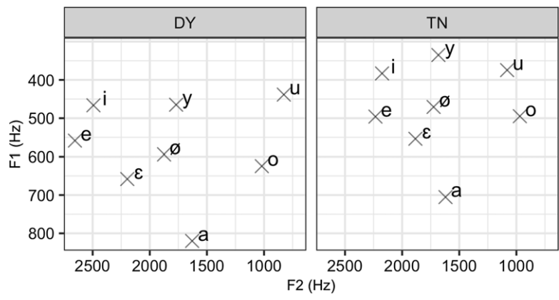
Figure 6. The acoustic vowel space of the eight short vowels (DY: left; TN: right). Each cross denotes the mean F1 and F2. The tokens for the formant frequency analysis are taken from the short vowel example list. The formant frequency values shown are averaged across all the data points of the vowel portion and across two repetitions of each token. The formant frequency is measured using the formant tracking algorithm implemented in PRAAT.
