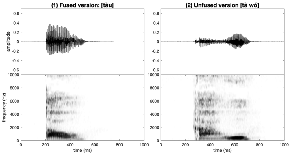
Figure 8. Examples of syllable fusion (data from DY). The waveforms and spectrograms illustrate the fused form [tàu] (left) and unfused form [tà wó] (right) of the word ‘spouse.’
