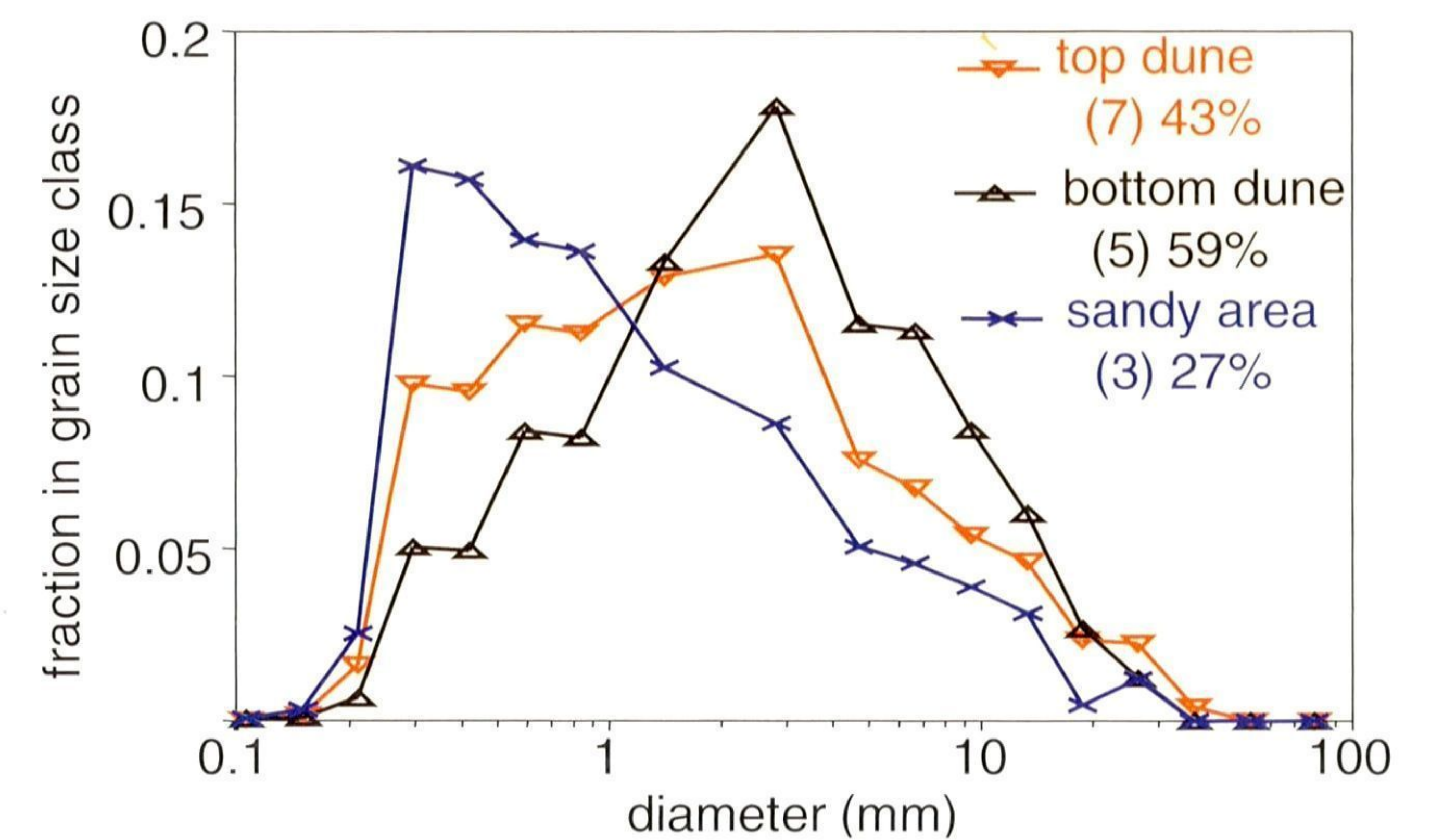
Fig. 6. Grain size distributions of selected samples of the sediment in the top and base of dunes in the Waal, and the fine surface sediment in the scour area of the Bovenrijn. Number of samples between brackets; gravel (>2 mm) percentage indicated.
