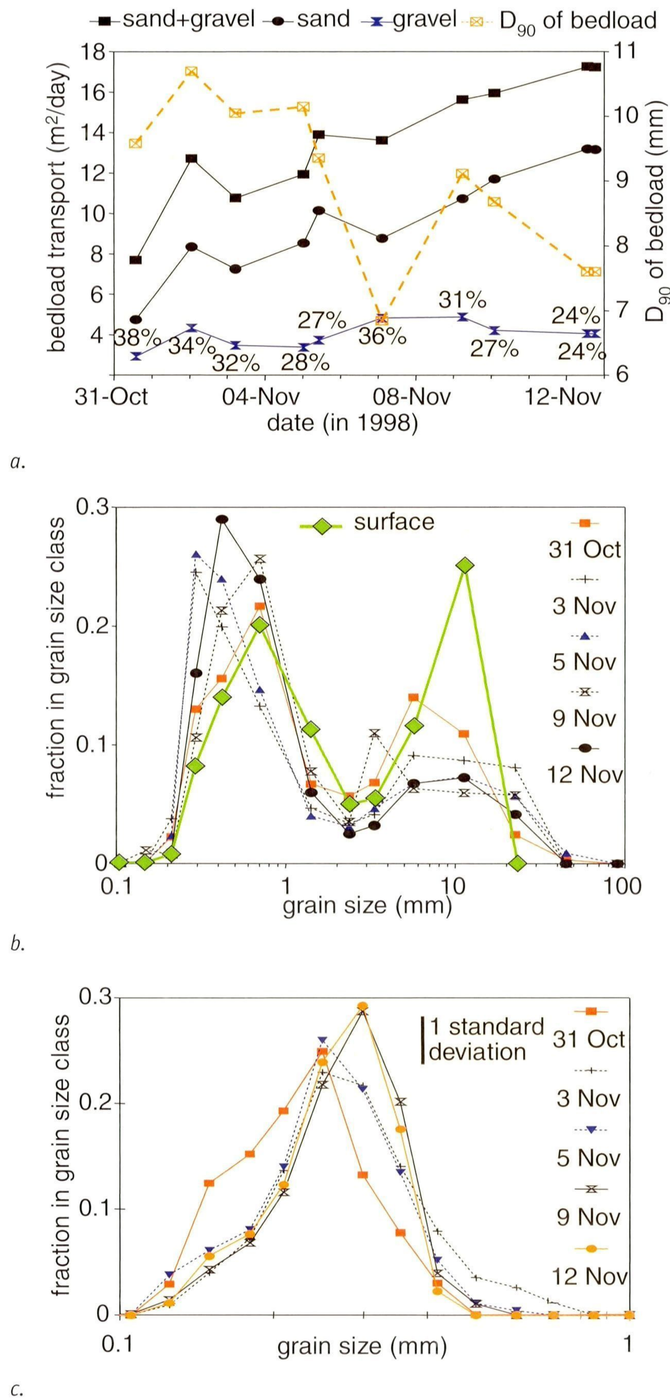
Fig. 5. a. Bedload transport in the river Waal by the HSZ, and the D 90 of the bedload sediment. The percentages refer to the precise gravel fraction. b. Grain size distributions of the bedload sediment. 'surface' refers to the surface bed sediment composition determined by Kleinmans & Ten Brinke (2001) (also shown in Fig. 2b). c. Grain size distributions of the suspended load sediment.
