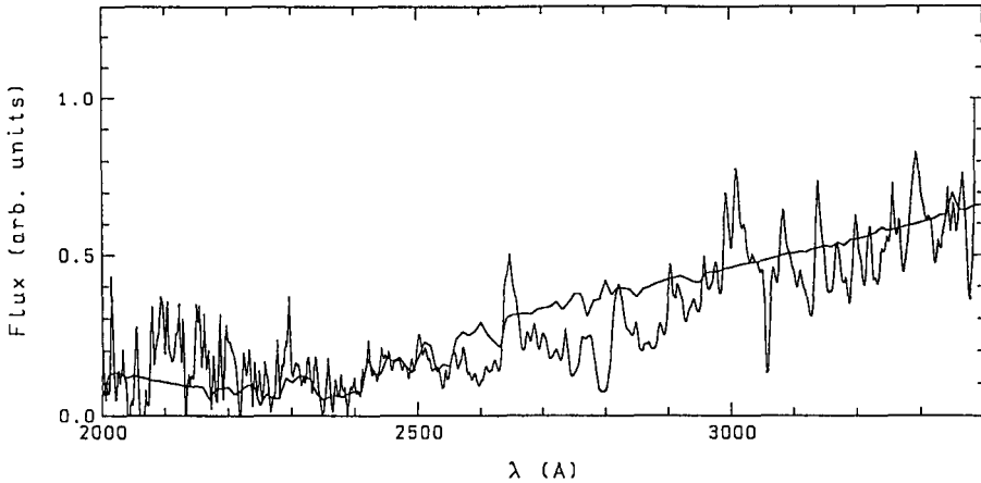
Figure 11. Comparison of the UV spectrum of the LMC nova 1988 no. 1 (Mar 29, 1988) (thin line) and a line-blanketed model with the parameters T_{eff} = 10^4 K, R_{\tau_{abs}=1} = 10^{11} cm, \rho_{out} = 2 \times 10^{-15} g cm ^{-3} and solar abundances (thick line).
