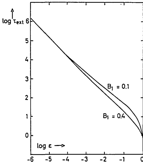
Figure 2. The optical depth in extinction where the local emissivity equals the emergent flux as a function of the ratio \epsilon = absorption coefficient / extinction coefficient for two values of the gradient of the Planck function.
