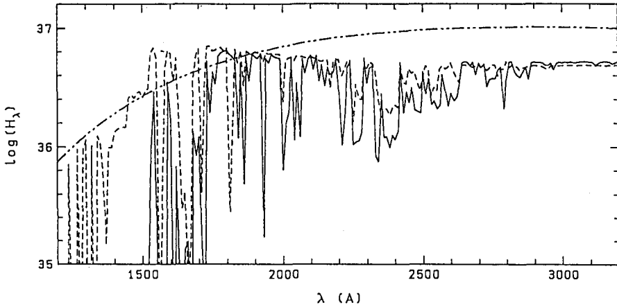
Figure 10. Effects of abundance changes on the UV spectra of novae: The broken curve shows the same blanketed flux distribution as Figure 8 whereas for the full curve an overabundance of all heavy elements by a factor of 5 is assumed. The dotted line again gives the black body spectrum.
