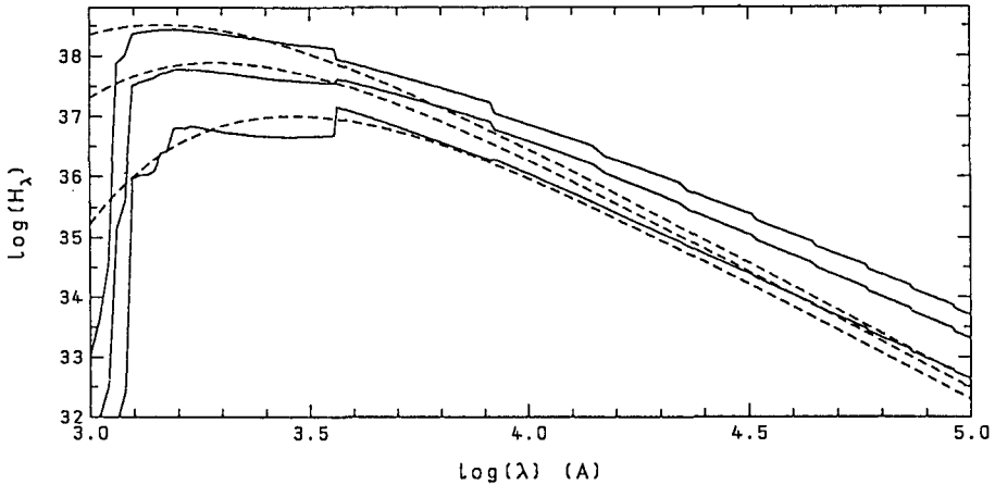
Figure 6. Continuum fluxes of nova photospheres (full curves) with R_{(\tau_{\text{abs}}=1)} = 10^{11} cm, outer densities \rho_{\text{out}} = 2 \times 10^{-15} \text{ g cm}^{-3} and effective temperatures T_{\text{eff}} = 10^4, 1.5 \times 10^4, and 2 \times 10^4 K from the ultraviolet to the infrared range. The broken lines give black body fluxes for the same temperatures.
