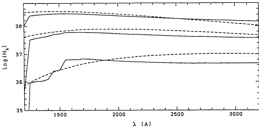
Figure 7. Same as Figure 6 but on an extended linear scale for the UV range.
