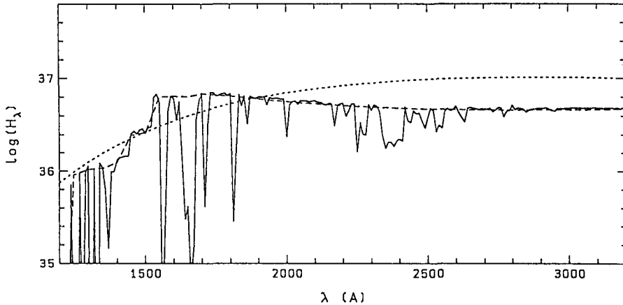
Figure 8. Comparison of the fluxes of a continuum model (broken curve) with a radius R(\tau_{abs} = 1) = 10^{11} cm, an outer density \rho_{out} = 2 \times 10^{-15} g cm^{-3} and an effective temperature T_{eff} = 10^4 K, of a metal line blanketed model (full curve) with the same parameters, and of a black body (dotted line) of the same temperature.
