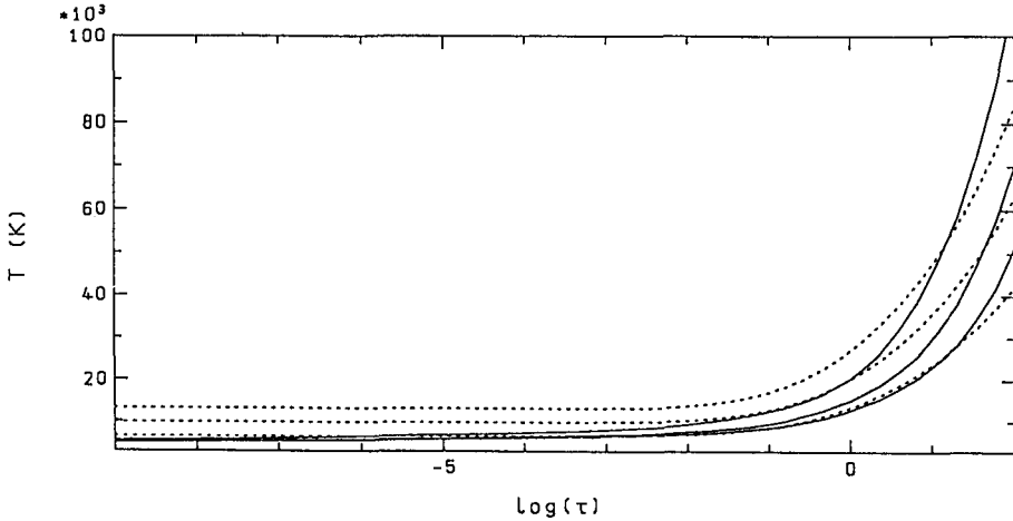
Figure 5. The temperature distributions in nova photospheres with R_{(\tau_{\text{abs}}=1)} = 10^{11} cm, outer densities \rho_{\text{out}} = 2 \times 10^{-15} \text{ g cm}^{-3} and effective temperatures T_{\text{eff}} = 10^4, 1.5 \times 10^4, and 2 \times 10^4 K. Also plotted are the corresponding grey distributions (dotted curves).
