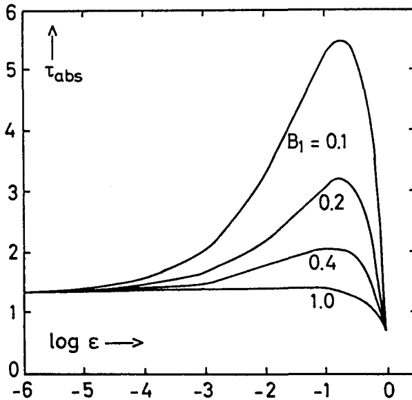
Figure 3. The optical depth in absorption where the local emissivity equals the emergent flux as a function of \epsilon . Note that the vertical axis is not logarithmic as in Figure 2 but linear.
