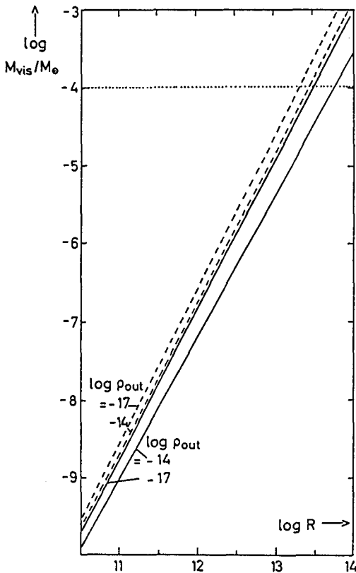
Figure 4. The mass M_{\text{visible}} visible to an observer for two values of the outer density. The full curves refer to an optical depth in scattering of unity, i.e. the volume between r_{\text{out}} and R , and the broken curves indicate masses up to the scattering optical depth
