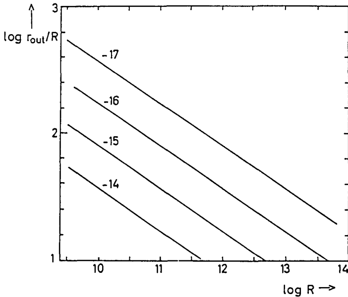
Figure 1. The relation between the outer radius r_{out} where the optical depth scale starts and the radius R where the optical depth in scattering is unity for different values of the density at r_{out} . The volume between r_{out} and R is directly accessible by spectroscopy since photons from it can reach the observer without interaction. It is seen that this volume is very much larger than the opaque core region.
