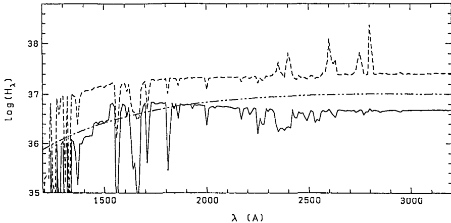
Figure 9. Demonstration of the significance of the temperature distribution in the outer layers: The full curve shows the same blanketed energy distribution as Figure 8 for which the temperature distribution of Figure 5 is used for all optical depths whereas for the broken curve it is assumed that the temperature distribution follows this run only up to \tau_{abs} < 10^{-4} and is constant for the upper layers.
