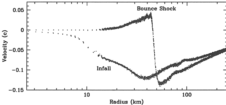
Figure 1. Velocity vs. radius plots of the collapse of a massive star before and just after the core reaches nuclear densities and bounces. This plots show a slice of the data from the 3-D simulations by Fryer & Warren (2002).
