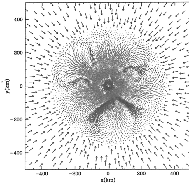
Figure 2. Upper panel: Diagram of the core of a massive star after bounce. In the center is the hot proto-neutron star above which is the convective region. Above the convective region, the rest of the star is falling down, forming a cap on the convective region. It is this cap that the neutrino driven pressure-cooker must overcome to drive an explosion. Lower panel: a slice of a 3-D simulation of this pressure-cooker (Fryer & Warren 2002).
