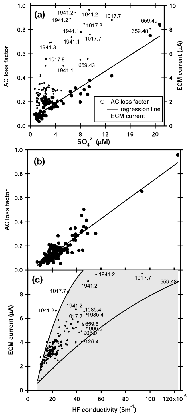
Fig. 3. Interrelations among the HF conductivities, AC loss factors, ECM signals and sulfate molarities. (a) AC loss factor (left axis) and ECM current (right axis) vs molarity of sulfate. Data points are from three portions indicated in Figure 1. More data points are shown than in Figure 2, because of another series chemical analysis not shown in Figure 2. For the ECM current, depths in meters for the larger values are labeled. (b) AC loss factor (left) vs HF conductivity (bottom). Data are from 167 depth points in the 2503 m Dome F ice core. The rightmost three data points are from the shaded parts in Figure 1. (c) ECM current (left) vs HF conductivity (bottom). 167 data points are from the same sample depths as used in (b). Distribution of the data points was emphasized by shading. Depths in meters for the larger values are labeled.
