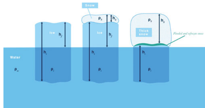
Fig. 1. Illustration of the mathematical components of sea-ice thickness measurement.
