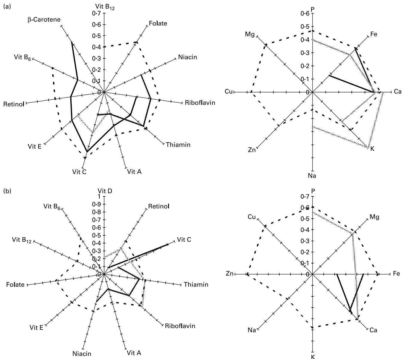
Fig. 3. Comparison of different dietary assessment methods in children (6–12 years) and adolescents (13–10 years) by vitamins and minerals (mean of quality weighted correlation coefficients) 24 HR, 24 h recall; EDR, estimated dietary record; WDR, weighed dietary record; DH, dietary history; YAQ, Youth/Adolescent Questionnaire. (a) Children (three or more studies: calcium, five studies FFQ v. 24 HR). —, FFQ v. EDR (three studies (26,31,36) ); - - - - -, FFQ v. WDR (two studies (16,23) ); ·····, FFQ v. BM (one study (35) ); - · - · - ·, 24 HR v. DH (one study (39) ); ■ - ■, YAQ v. 24 HR (one study (29) ); - · - · - ·, FFQ v. 24 HR (five studies (11,13,16,25,38) ). (b) Adolescents (three or more studies: calcium: three studies FFQ v. 24 HR; three studies FFQ v. WDR). —, FFQ v. 24 HR (three studies (11,14,20) ); - - - - -, FFQ v. WDR (three studies (16,27,33) ); - · - · - ·, 24 HR v. DH (one study (39) ); ■ - ■, YAQ v. 24 HR (one study (29) ).
