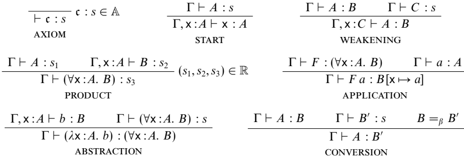
Fig. 1. Typing rules of PTS with specification (\mathbb{S}, \mathbb{A}, \mathbb{R}) .
