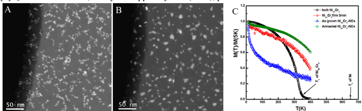
Figure 1. Annular dark field STEM images were acquired at 300kV. The images were taken at room temperature (A) before and (B) after annealing at 550 °C. (A) Shows the as grown \text{Ni}_{95}\text{Cr}_5 NCs with an average size of 6nm. (B) Shows the same area as (A) after annealing the sample at 550 °C. The NCs undergo coalescence (e.g. red squares) and present a wider size distribution with an average size of 11 nm. (C) Normalized magnetization curves vs. temperature for the as-grown and annealed NCs, as well as for a \text{Ni}_{95}\text{Cr}_5 thin film and bulk \text{Ni}_{95}\text{Cr}_5 for comparison.
