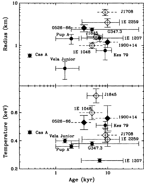
Figure 1. Age dependences of BB radius and BB effective temperature for CCOs (filled circles), AXPs (open diamonds) and SGRs (filled diamonds). For objects with known SNR association, estimated SNR ages are used (solid horizontal error bars) while for four magnetars (marked with horizontal dash lines) we use spin-down ages.
