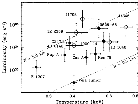
Figure 2. The dependence of bolometric BB luminosity on BB temperature (Hertzsprung-Russell diagram) for CCOs and magnetars. The lines of constant BB radius are plotted at 0.3 km and 3.0 km.
