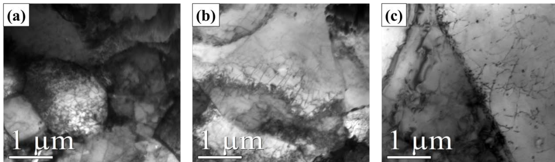
Figure 1. TEM images of dislocation structures of the steel after piping process: (a) near surface, (b) one quarter, and (c) center of the sample
