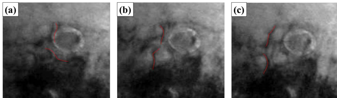
Figure 2. TEM images captured during the in-situ straining. Dislocations (marked as red lines) were gradually unpinned from the precipitate under continuous loading.
