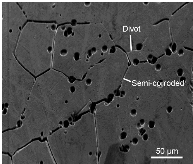
Figure 2: A SEM image showing the semi-corroded boundaries and asymmetrical divot-like features.
