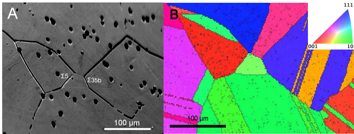
Figure 1: (A) A SEM image showing preferentially corroded grain boundaries and different grain boundary geometry. (B) The corresponding EBSD map showing the crystallographic orientations of the grains in order to determine grain boundary geometry.
