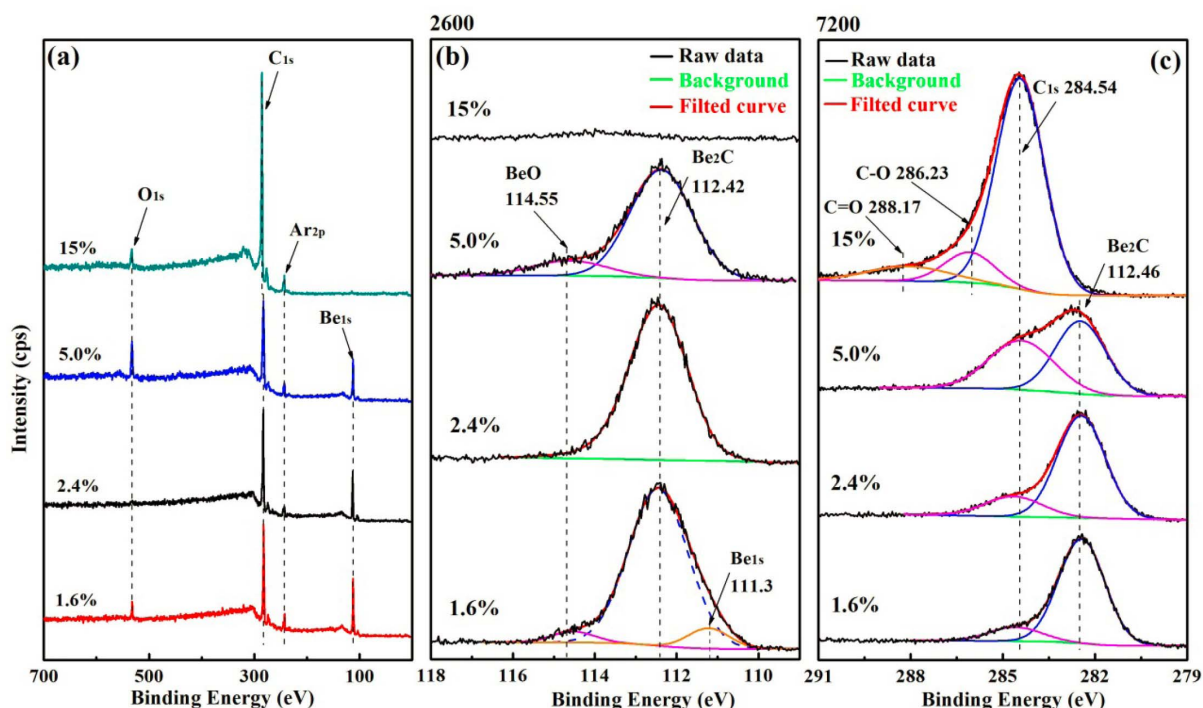
Figure 3. XPS spectra for films prepared at different \text{CH}_4 -Ar ratios after 30 min \text{Ar}^+ etching survey spectrum (a), deconvolution of \text{Be}1s peaks (b) and deconvolution of \text{C}1s peaks (c).
