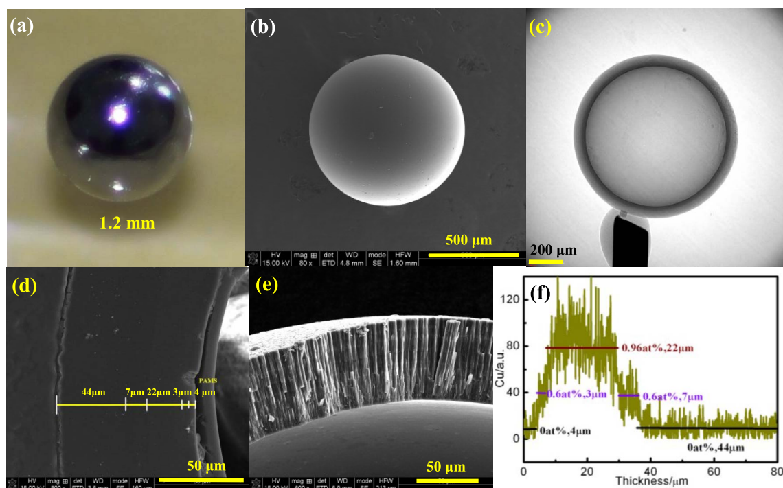
Figure 1. Be–Cu capsule. (a) Optical microscope image, (b) SEM image, (c) micro-CT image, (d) polished cross-section morphology, (e) cross-section morphology, (f) Cu dopant distribution at cross-section.
