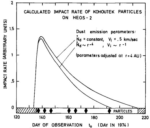
Fig. 2: Effect of varying dust emission rate \dot{N}_d and varying emission speed v_i on the impact rate.
