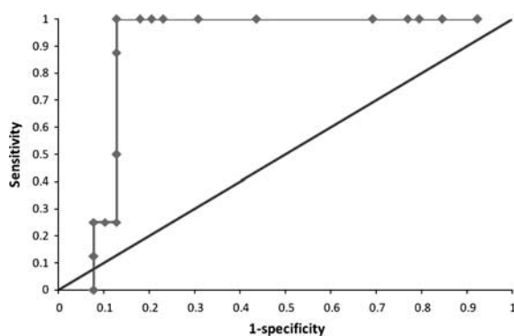
Figure 1 Area under the receiver operator characteristic (ROC) curve for the 30-item Geriatric Depression Scale to identify depression, according to a diagnostic assessment using ICD-10 criteria
