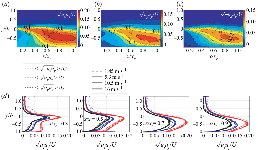
Figure 4. Reynolds stress statistics in the shear layer. Contours of: (a) \sqrt{u_x u_x} / U , (b) \sqrt{u_y u_y} / U and (c) \sqrt{-u_x u_y} / U at U = 16 \text{ m s}^{-1} . (d) Wall-normal profiles at the indicated streamwise locations, and at four different speeds.
