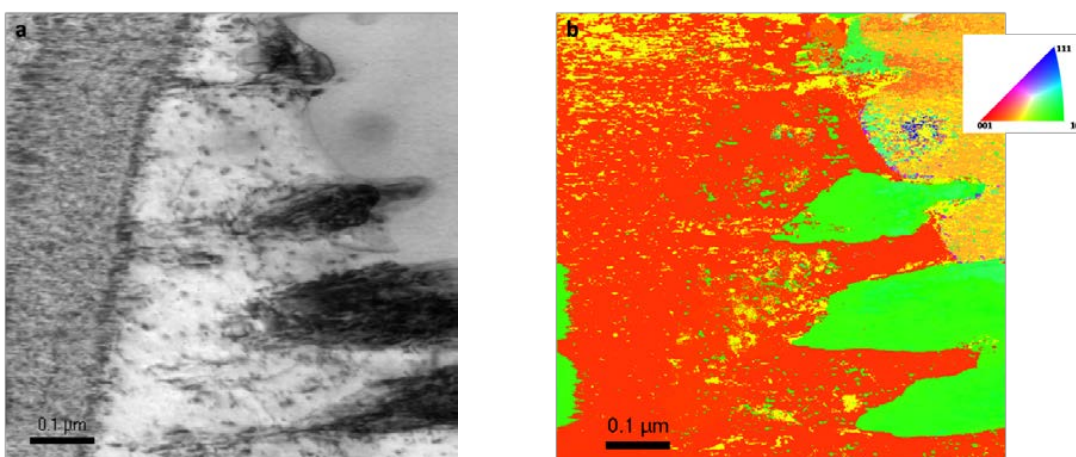
Figure 3 – NBD in a sample aged at 650°C for 60min. (a) Reconstructed bright field image. Notice the DC colonies, with precipitates with dark contrast. (b) Crystallographic orientation map.
