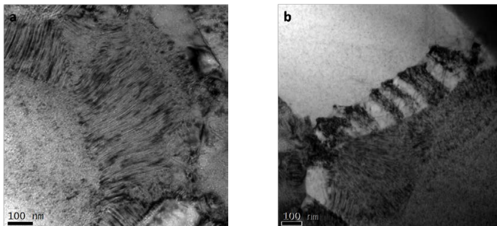
Figure 1 – TEM bright field images. (a) DP colony in sample aged at 550°C for 60min. (b) Discontinuous coarsening after 30min at 550°C.
