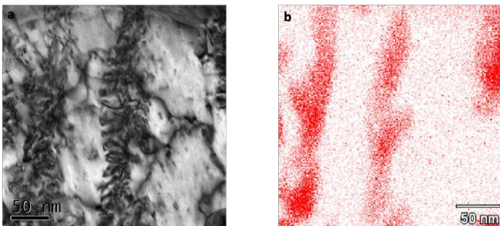
Figure 2 – (a) TEM bright field of semi-coherent DC after 60min at 650°C. (b) Corresponding EDS Co mapping.
