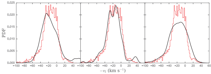
Figure 2. Distribution of v_l ( \text{km s}^{-1} ) at (l, b) = (180, 0) \pm 5 deg (red) overlaid with three model predictions (black), originally shown in Hunt et al. (2017).
