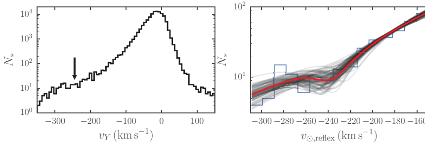
Figure 1. Left: Distribution of tangential velocities, v_Y ( \text{km s}^{-1} ), with a ‘dip’ visible around v_Y = -240 \text{ km s}^{-1} , marked with an arrow. Right: Tail of the v_Y distribution overlaid with the best-fit model (red), and 100 MCMC samples (black). As shown in Hunt et al. (2016).
