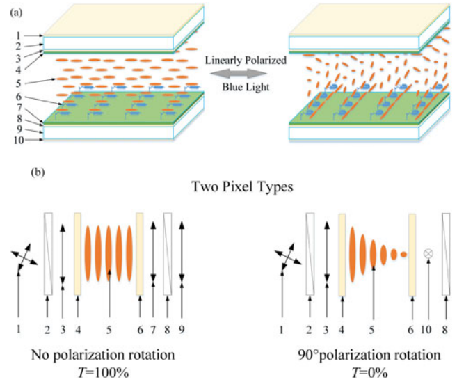
Figure 1. (a) Structure of the LC binary mask (1 – anti-reflection coating, 2 – front glass substrate, 3 – anti-reflection coating, 4 – polyimide layer, 5 – LC molecule, 6 – azobenzene group, 7 – photoalignment layer, 8 – anti-reflection coating, 9 – rear glass substrate and 10 – anti-reflection coating) and (b) arrangement of LC molecules in a single pixel of two pixel types (1 – incident light, 2 – polarizer, 3 – P-polarized light, 4 – front glass substrate with coating polyimide, 5 – LC molecule, 6 – rear glass substrate with coating azobenzene, 7 – P-polarized light, 8 – polarizer, 9 – output light and 10 – S-polarized light).
