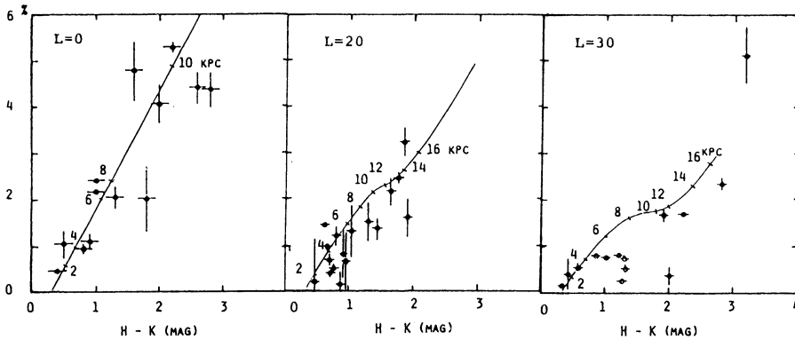
Figure 2. H - K dependence of the observed polarization in 3 longitude regions. The expected dependences are shown by curves, with distance scales estimated from the HI and CO data.
