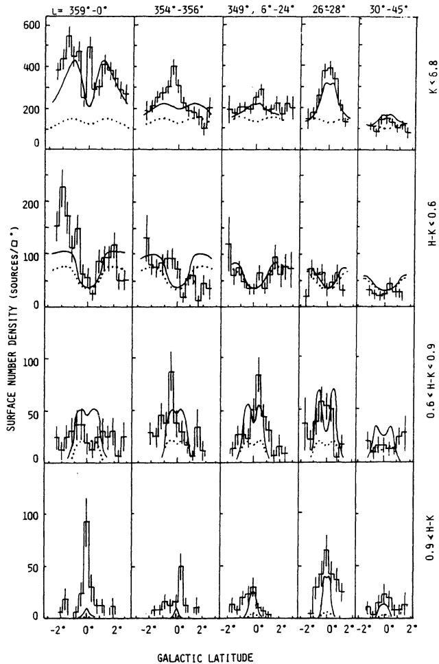
Figure 1. Surface density of infrared sources as a function of galactic latitude in various longitude intervals (top scale). Uppermost panels: total numbers of bright infrared sources. Other panels: distributions for sources in various infrared-colour ranges. Dotted and solid lines represent model calculations (see text).
