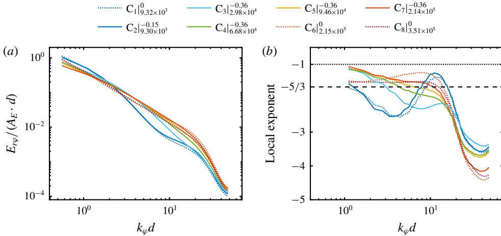
FIGURE 14. (a) Temporally and azimuthally averaged azimuthal kinetic energy co-spectra evaluated at \tilde{r} = 0.5 . Spectra are normalized to cover an area of 1 under their respective curves and by the gap width d . (b) Local scaling exponent \gamma of the co-spectra for E_{r,\varphi} \sim k_\varphi^\gamma calculated with a bin size of \log_{10}(k_\varphi) = 0.5 . Legend abbreviations represent C_{\#} |_{Re_S}^\mu .
