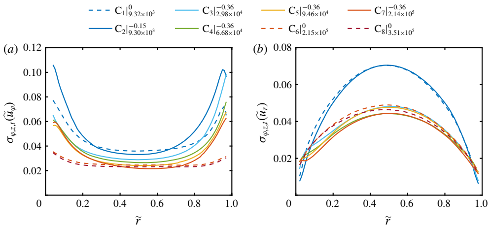
FIGURE 5. Radial profiles of the standard deviation of the (a) azimuthal and (b) radial velocity component, calculated over space (cylindrical surfaces) and time. The profiles are normalized by the shear velocity u_s . Legend abbreviations represent C_{\#}|_{Re_S}^\mu .
