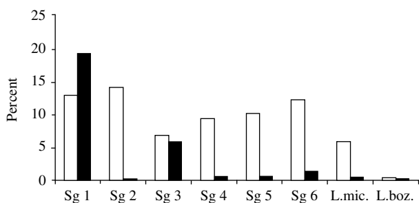
Fig. 3. Legionella seroprevalence in the study population (□) compared to the distribution of species and serogroups isolated from cases of Legionnaires' disease (■) in the Danish population [seroprevalence defined as titres of at least 1:128 in 2004]. Legionnaires' disease 1994–2004 ( n=1004 ), notified to the Department of Epidemiology, Statens Serum Institut, according to the known specified species and serogroups ( n=313 ). L.mic, Legionella micdadei ; L.boz, Legionella bozemanii .
