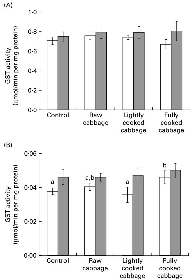
Fig. 2. Specific activity of glutathione-S-transferase (GST) in rat (A) liver and (B) colon, expressed as \mu\text{mol S-2,4-dinitrophenylglutathione} formed/min per mg cytosolic protein, after consumption of a control diet or diets containing raw, lightly cooked or fully cooked cabbage by germ-free ( \square ) and human faecal microbiota-associated ( \blacksquare ) rats. Values are means of six replicates, with standard errors represented by vertical bars. a,b Mean values for the GF rats with unlike letters were significantly different ( P < 0.05 ). Liver GST was not influenced by cooking treatment applied to cabbage, or microbiota status. Colonic GST was affected by dietary treatment in germ-free rats only ( P < 0.05 ).
