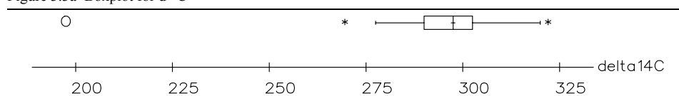
Figure 3.3b Boxplot for D 14 C
