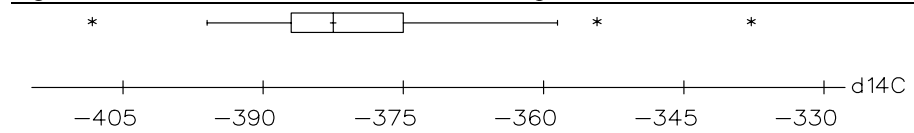
Figure 3.4 Distribution of results TIRI D: Hekla peat
