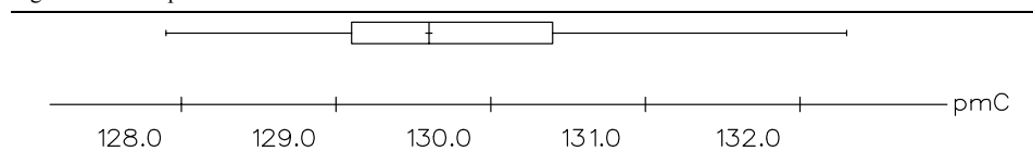
Figure 3.3c Boxplot for pMC
