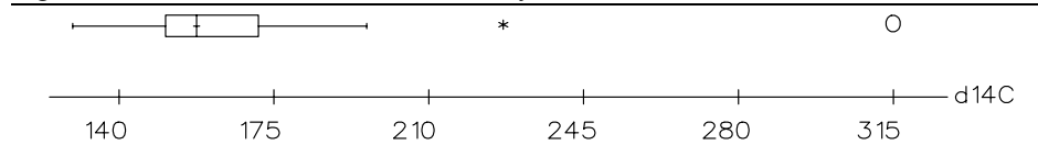
Figure 3.1a Boxplot for d^{14}C
