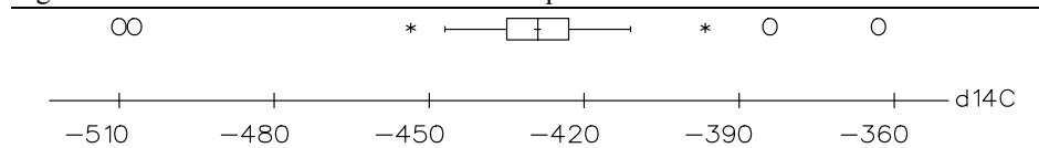
Figure 3.2a Boxplot for d^{14}C
