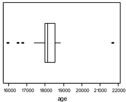
Figure 4.5 Distribution of age for TIRI-K
