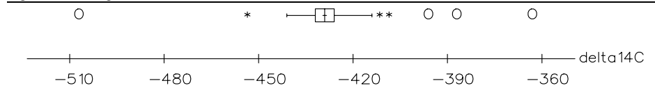
Figure 3.2b Boxplot for D^{14}C
