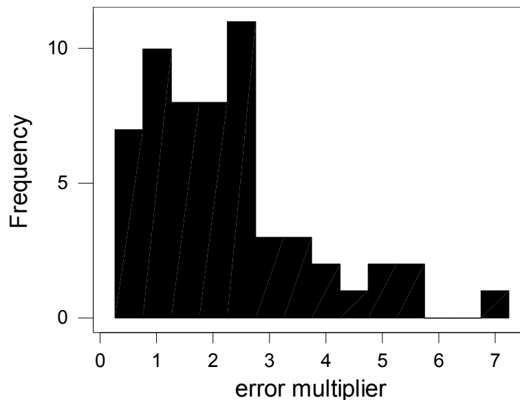
Figure 5.1 Histogram of error multipliers
