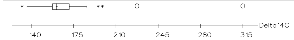
Figure 3.1b Boxplot for D^{14}C
