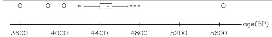
Figure 3.2c Boxplot for age (yr BP)
