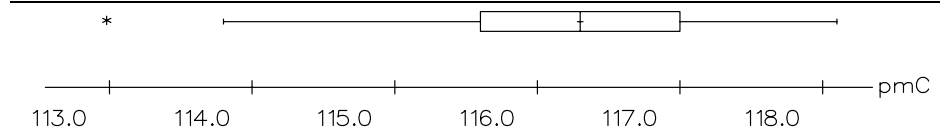
Figure 3.1c Boxplot for pMC
