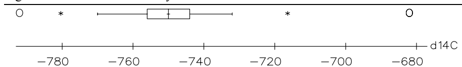
Figure 3.5 Statistical summary for TIRI E: Ellanmore humic
