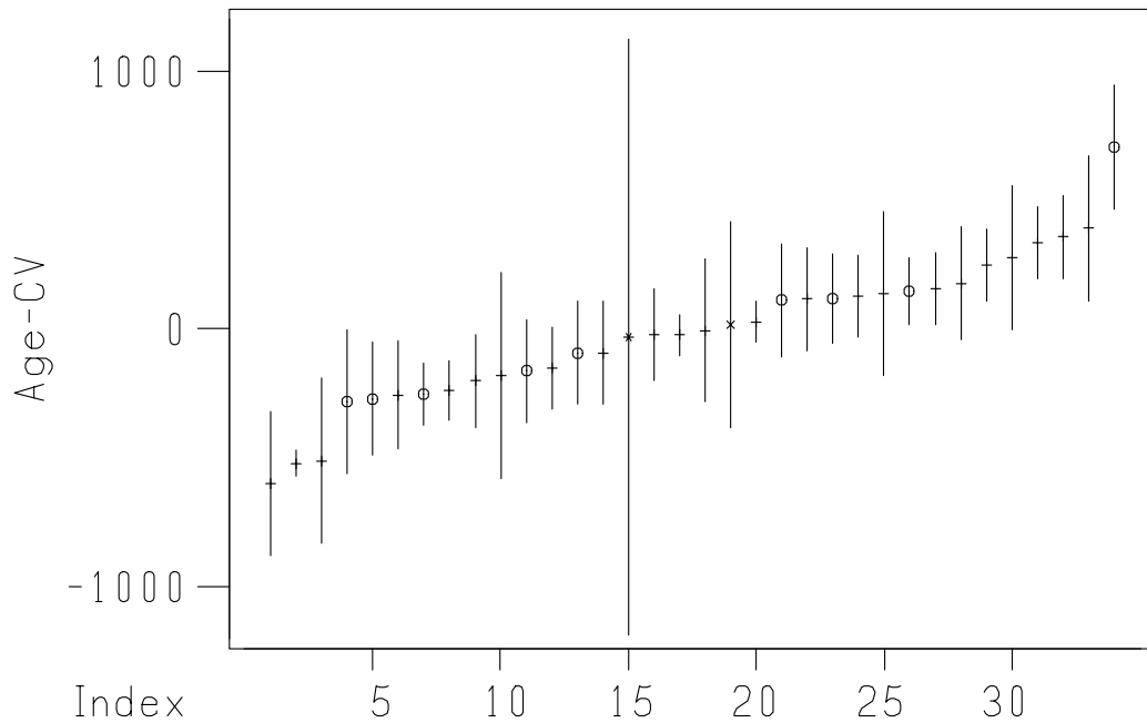
Figure 4.9 Sample H: Ellanmore peat
