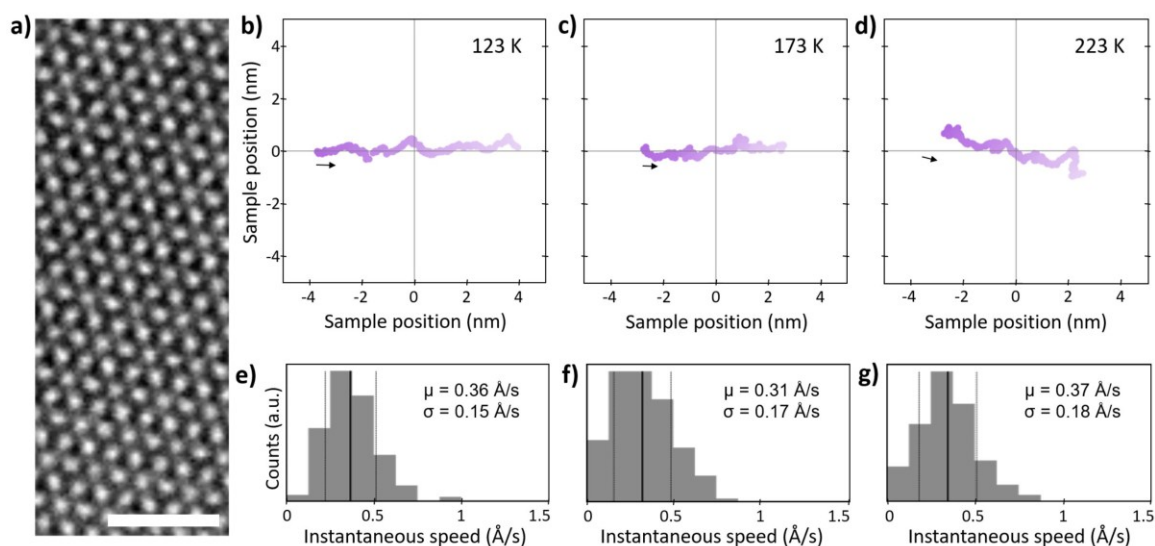
Figure 1. Figure 1. Stable high-resolution imaging at intermediate temperatures. (a) Atomic-resolution HAADF-STEM image of Nb 3 Br 8 at \sim 223 K. Scale bar=1 nm. Drift performance of the continuously variable temperature cryo-STEM holder at various low temperatures measured by sample positions plotted over a time of 250 s at (b) 123 K, (c) 173 K, and (d) 223 K. (e-g) Corresponding instantaneous drift speed histograms. Mean speed ( \mu ) and standard deviations ( \sigma ) marked by solid and dotted vertical lines, respectively. Figure adapted from reference [10].
