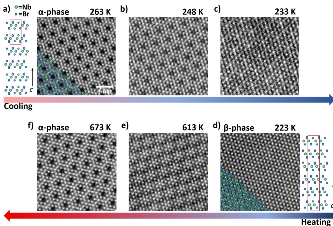
Figure 2. Figure 2. Atomic-scale visualization of a phase transition at intermediate temperatures. Plan-view HAADF STEM images of (a) \alpha -Nb 3 Br 8 at 263 K, (b) an intermediate phase at 248 K, (c) a disordered transition phase at 233 K, (d) \beta -Nb 3 Br 8 at 223 K, (e) an intermediate phase at 613 K, and (f) recovery of \alpha -Nb 3 Br 8 at 673 K. Images were taken sequentially on the same flake during temperature cycling in a single experiment. Predicted \alpha -Nb 3 Br 8 and \beta -Nb 3 Br 8 structures as viewed down the c axis are overlaid on corresponding images and models of cross-section views are shown next to each image (red box denotes the unit cell). Scale bar=1 nm; all images are same scale.
