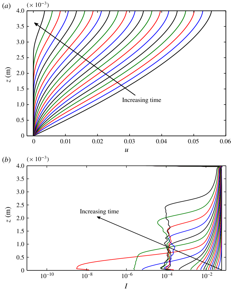
FIGURE 3. Downslope averages of the velocity (a) and the inertial number (b) at evenly spaced times in 0 < t < 0.2 s. Here the computation is initialised with the Bagnold solution (5.4) and (5.5) with \zeta_0 = 24^\circ and the fields are computed with the Jop et al. (2005) rheology (2.12). The slope angle during the computation is \zeta = 10^\circ and the numerical grid is 256 \times 256 cells with a time step 1 \times 10^{-6} s.
