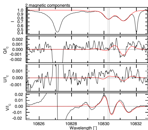
Figure 1. Profile showing 2 magnetic components (observed profile: black, fitted profile: red). Fit parameters for fast component: \gamma = 65^\circ , B = 640 G; component at rest: \gamma = 26^\circ , B = 470 G
