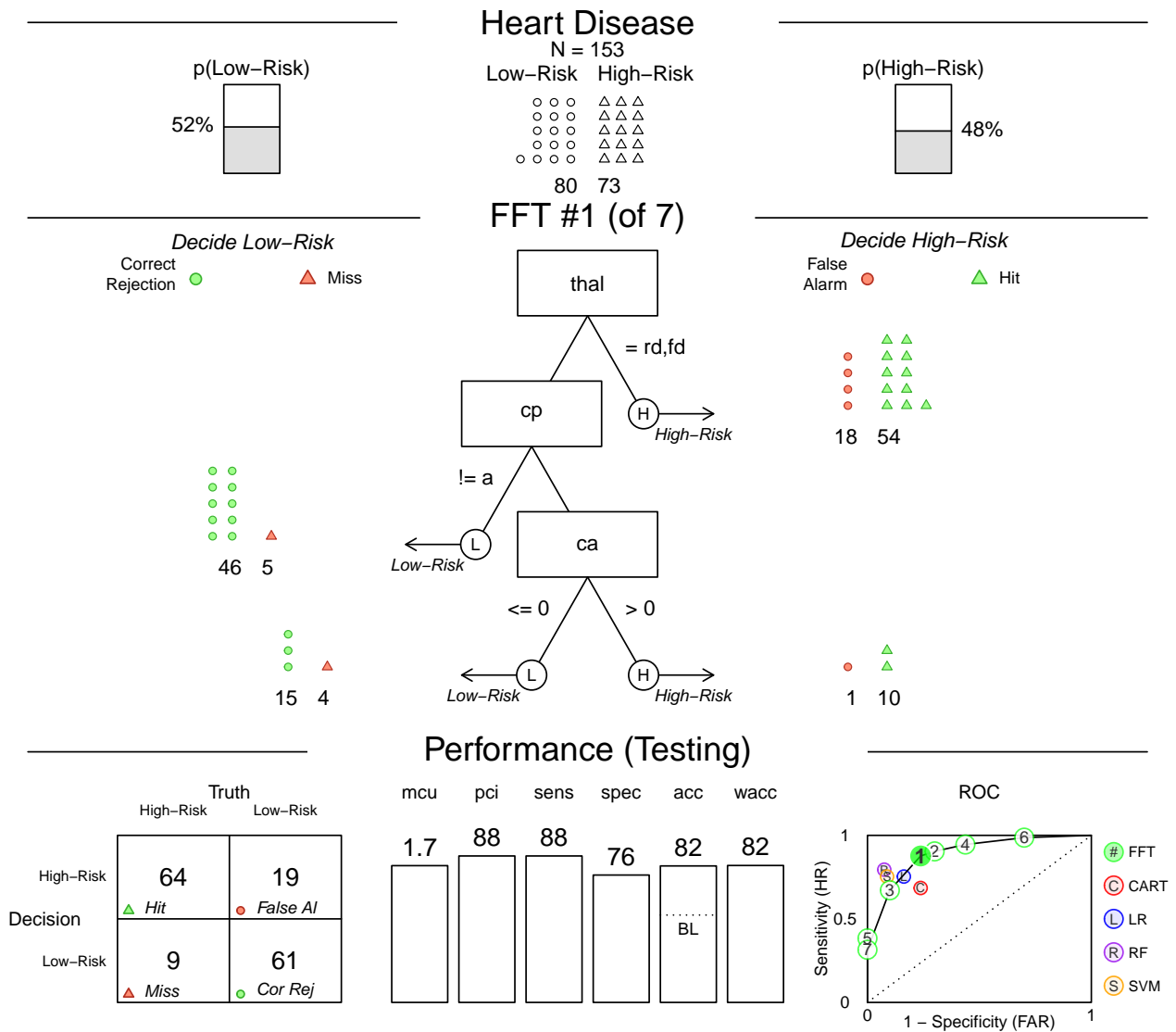
FIGURE 6: Visualization of an FFTrees object created by plot(heart.fft, data = "test"). The top panel shows information about the dataset, including the frequencies and base rates of negative and positive criterion classes. The middle panel contains the FFT and icon arrays showing the the number and accuracy of cases classified at each node. This particular FFT's interpretation has been described above (on p. 346 and in Figure 2). The bottom panel shows the FFT's cumulative classification performance, including a confusion table and levels for a range of statistics. The bottom right plot shows the performance of all seven FFTs created by the FFTrees() function in ROC space (green circles with numbers correspond to FFTs). The FFT currently being plotted is highlighted (here, FFT #1, with the highest weighted accuracy in training). Additional points in this plot correspond to the performance of competing classification algorithms (see Simulation section): standard decision trees (CART), logistic regression (LR), random forests (RF), and support vector machines (SVM). In this case, FFT #1 has a higher sensitivity than competing algorithms, but at the cost of a lower specificity. Additionally, FFT #1 dominates CART in this example by having a higher sensitivity and comparable specificity.
