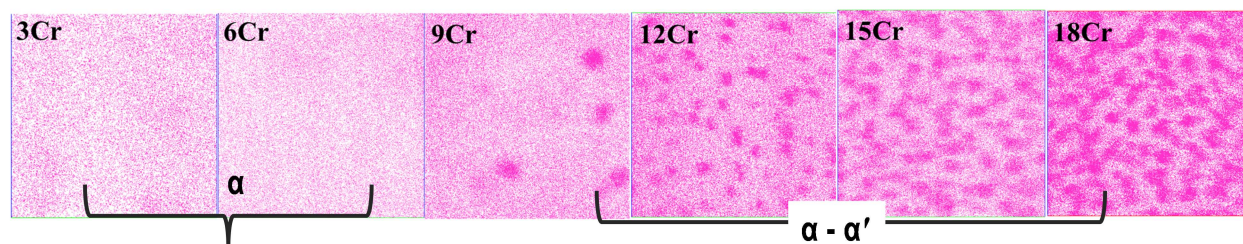
Figure 1: 20 nm thick slices showing the distribution of Cr atoms for each of the analyzed alloys: (a) Fe-3Cr, (b) Fe-6Cr, (c) Fe-9Cr, (d) Fe-12Cr, (e) Fe-15Cr, (f) Fe-18Cr
