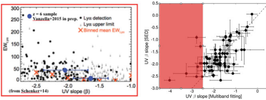
Figure 3. Left: Relation between UV \beta slope and the Ly \alpha equivalent width from Schenker et al. (2014). We report the \beta slope and EW(Ly \alpha ) derived from the stacked spectra for LAEs and non LAEs (blue dots). Right: Comparison between UV \beta slopes derived from multiband fitting of the photometry (Castellano et al. 2012) and UV \beta slopes derived from SED fitting. The red region indicates observed UV slopes bluer than theoretically expected (see Text).
