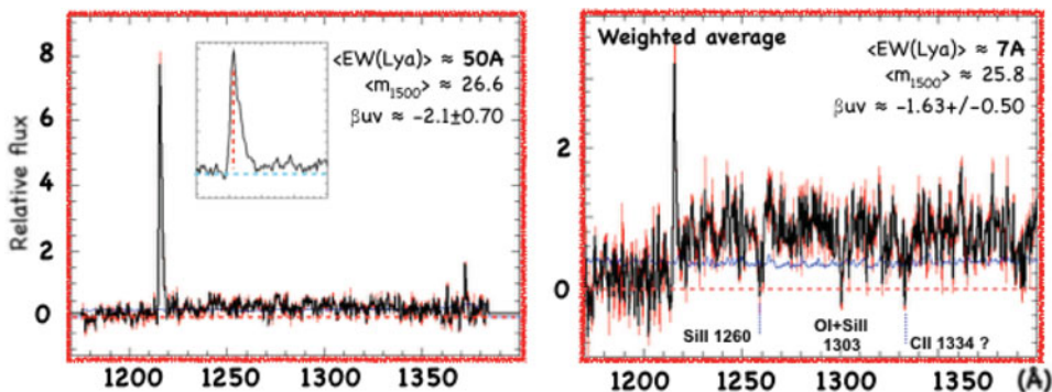
Figure 2. Stacking of VLT/FORS2 spectra for z \sim 6 LAEs (left) and non LAEs (right). Some interstellar medium lines are visible in the stacked spectrum of non LAEs.
