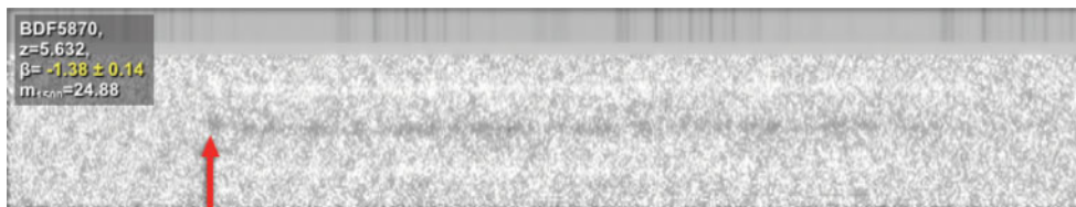
Figure 1. Two-dimensional VLT/FORS2 spectrum of a z = 5.632 non Lyman- \alpha emitter. While there is no line detected, the observation is deep enough to detect the continuum. The red arrow shows the Lyman break.
