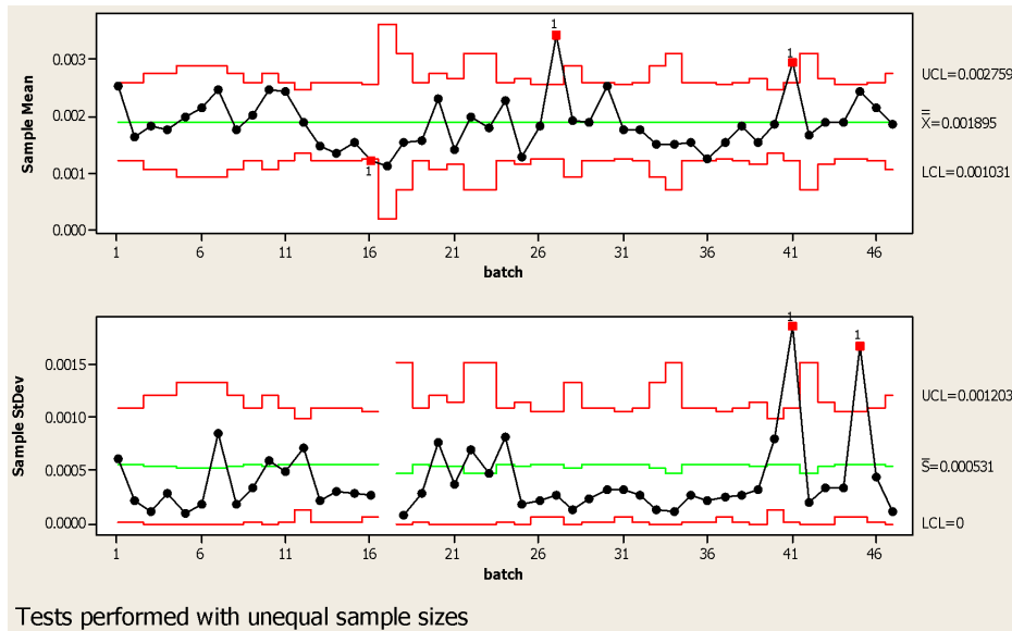
Figure 4 Control chart for wheels run on both machines showing results for a background standard (BK-HW)
