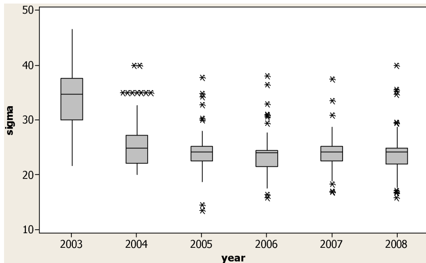
Figure 2 Boxplot of the 1- \sigma data for Belfast cellulose from 2003 to 2008
